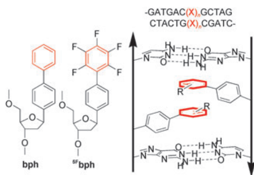
Figure 1. Chemical structures of the biaryl nucleoside analogues investigated, and the proposed interstrand stacking recognition motif of such aromatic units ( X ) in the center of an oligodeoxynucleotide duplex with the indicated sequence.
