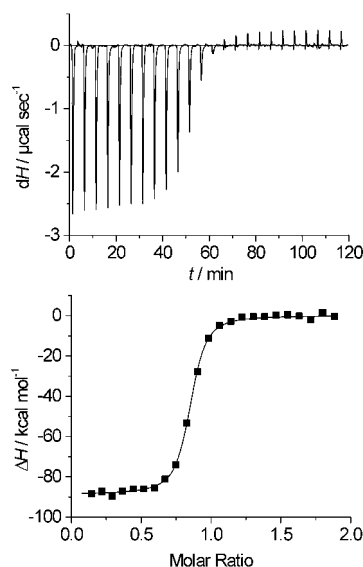
Figure 2. Isothermal titration calorimetry ( T = 301.4 K). Top: heat signal versus time for the titration of d(GATGAC(bph) 3 GCTAG) ( c = 10.0 \mu\text{M} ) with d(CTACTG(bph) 3 CGATC) ( c = 99.8 \mu\text{M} ) in NaH 2 PO 4 (10 mM), NaCl (150 mM), pH 7.0; bottom: corresponding normalized heat signal versus molar strand ratio.
