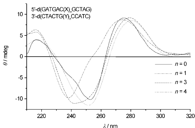
Figure 3. CD spectra of duplexes containing 0–4 5 Fbph base-pairs ( X = Y = ^5\text{Fbph} ); c = 3.6 μM in NaH 2 PO 4 (10 mM), NaCl (150 mM), pH 7.0, T = 20 °C.
