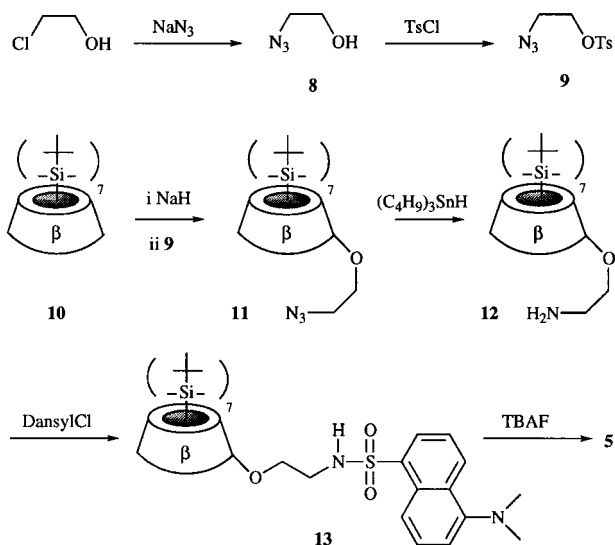
Scheme 1 Synthesis of 5
