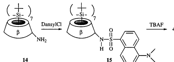
Scheme 2 Synthesis of 4
