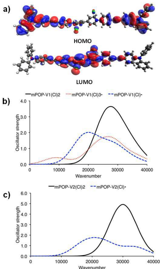
Figure 1 a) DFT HOMO and LUMO of mPOP-V1(Cl) 2 and computed [TDA-BMK/6-31G(d)] UV/Vis spectra for the model systems b) mPOP-V1 and c) mPOP-V2.
