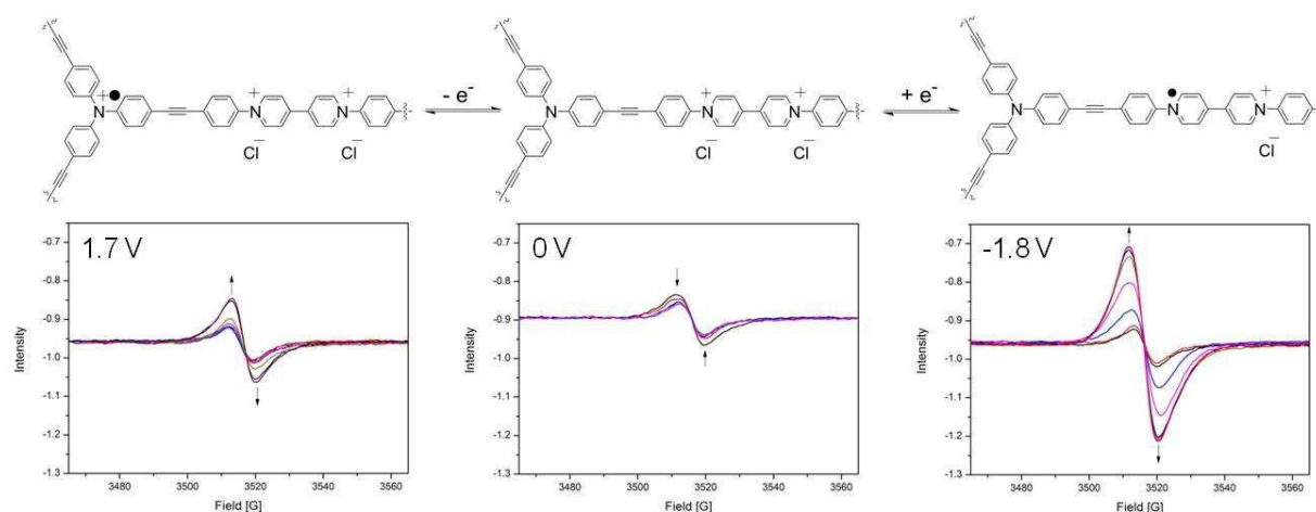
Figure 4. Solid state EPR spectroelectrochemical data for POP-V1 in [(n\text{-C}_4\text{H}_9)_4\text{N}]\text{PF}_6/\text{CH}_3\text{CN} electrolyte. The arrows indicate the direction of spectral progression throughout the course of the experiment.
