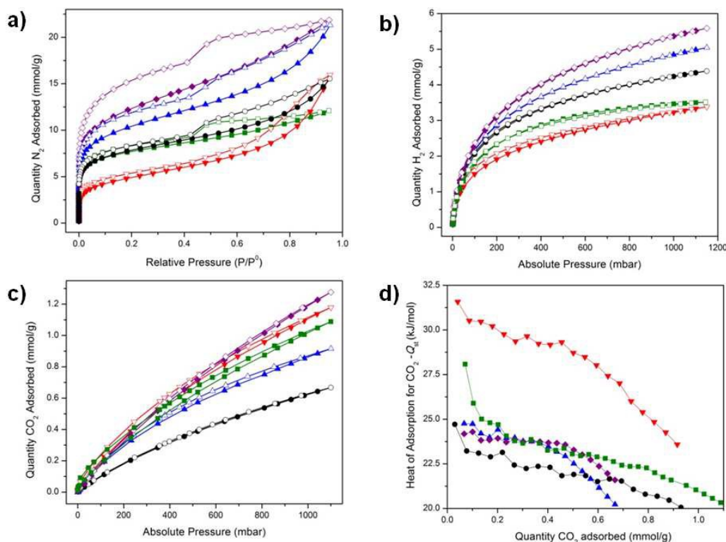
Figure 5. Gas sorption isotherms of POP-V1 (▲), ox-POP-V1 (▼), red-POP-V1 (○) and POP-V2 (◆), red-POP-V2 (■) for a) N 2 at 77 K, b) H 2 at 77 K, c) CO 2 at 298 K and d) the isosteric heat of adsorption for CO 2 where adsorption = filled symbols and desorption = open symbols. The lines joining each point are provided as a guide to the reader.
