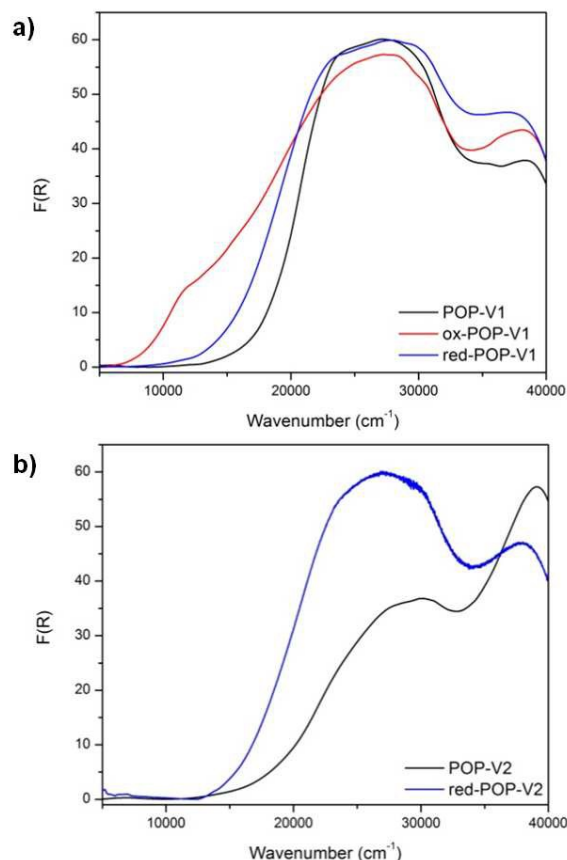
Figure 2 Solid state UV/Vis/NIR spectra of a) POP-V1, ox-POP-V1 and red-POP-V1, b) POP-V2 and red-POP-V2 over the range 5000-40000 cm -1 .
