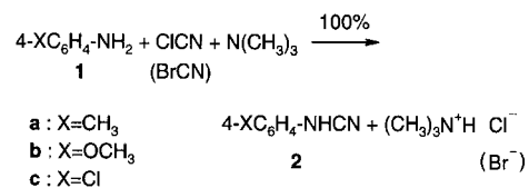
Scheme 1. Gas–solid synthesis of cyanamides from primary amines and ClCN or BrCN.
