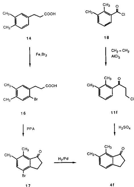
Scheme 3
