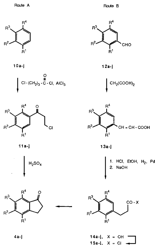
Scheme 2
