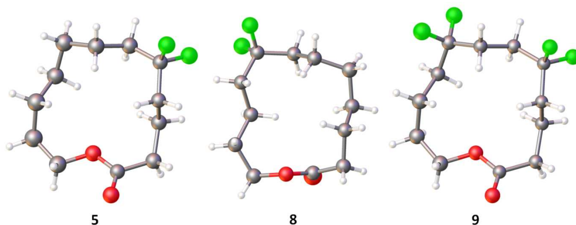
Fig. 1 Representations of the X-ray derived structure of 12-dodecanolides 5 , 8 and 9 . In all cases the CF 2 groups adopt corner locations in the solid state.
