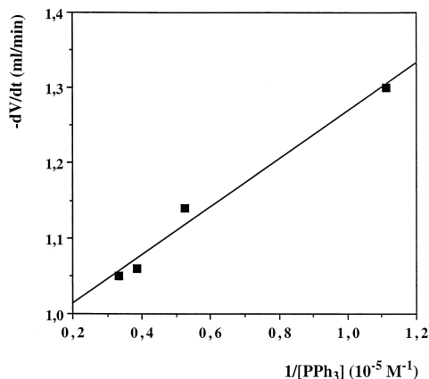
Fig. 2. Plot of the rate of hydrogenation of phenylacetylene to styrene versus 1/[PPh_3] in dichloromethane at 25^\circ\text{C} , 1 atm H_2 , 1.55 \times 10^{-3} M [Catalyst], 0.067 M PhC_2H .
