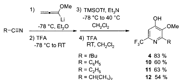
Scheme 6.
