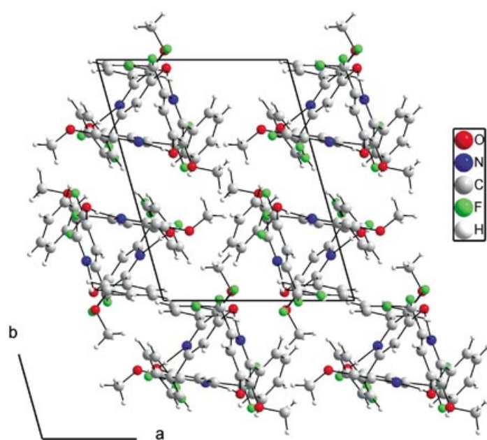
Figure 2. Packing of 10 along the c axis.
