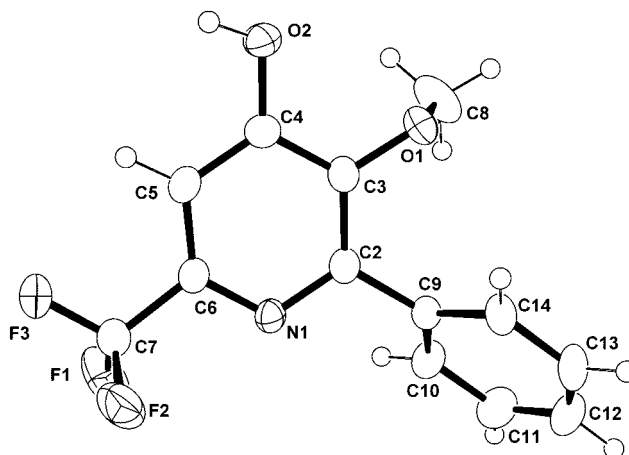
Figure 1. Structure of 10 (ORTEP plot; 50 % probability level).
