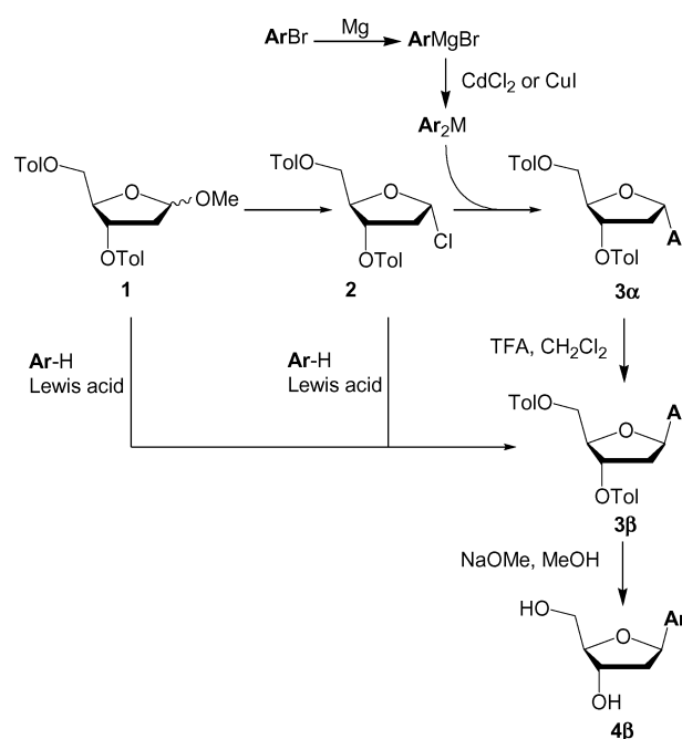
Scheme 1 Comparison of aryl C -nucleoside synthesis by organometal reagents with Friedel–Crafts alkylation. (M = Cd or CuMgX, Tol = toluoyl, X = halide).
