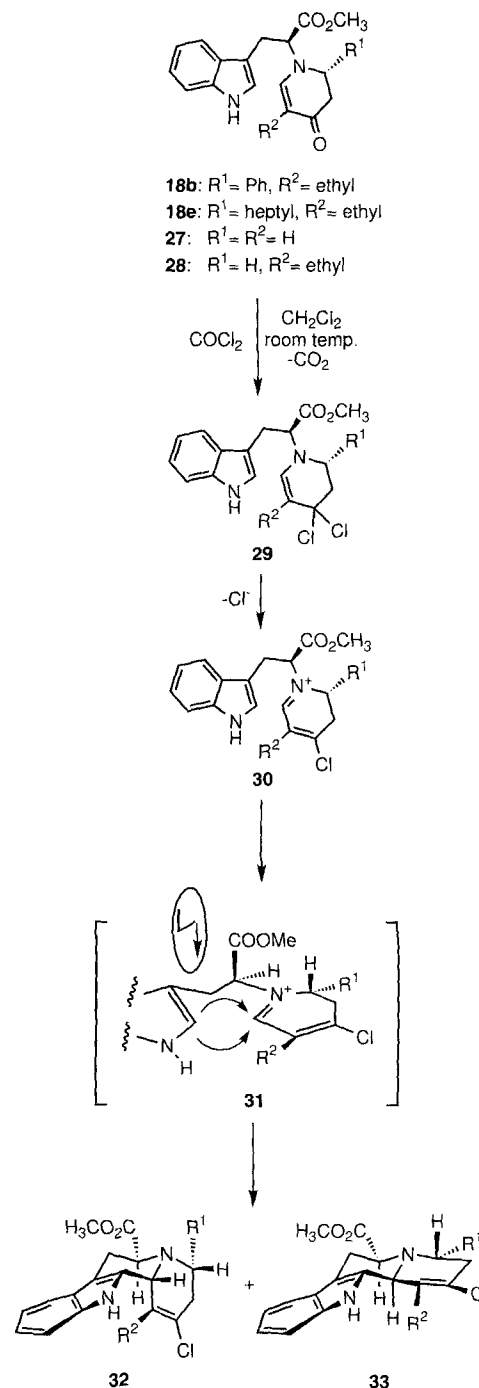
Scheme 5. Cyclization of the diidehydropiperidine-4-ones 18 to indolo[2,3- a ]quinolizines.
