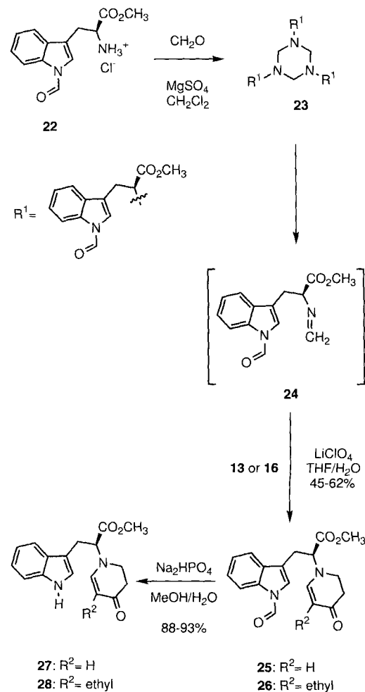
Scheme 4. Tandem Mannich–Michael reactions employing the formalimine 24 of tryptophan methyl ester.
