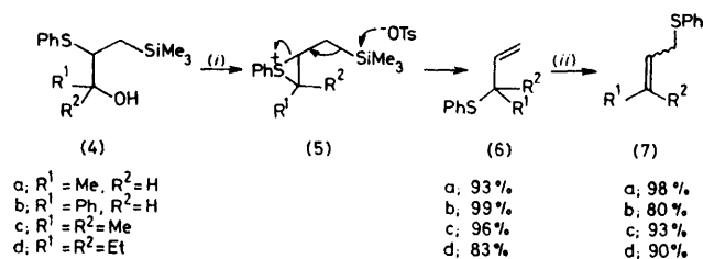
SCHEME 1 (i) TsOH-C 6 H 6 reflux (secondary alcohols) or TsOH-MeCN-20 °C (tertiary alcohols); (ii) sunlight-CCl 4 , 20 °C
