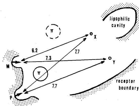
Figure 2. The topography of the dopamine receptor. P and M are putative binding sites on the receptor surface complementary to the p -OH and the m -OH groups of the agonist molecule; X and Y are putative electronegative binding sites complementary to a nitrogen atom of the agonist. Areas indicated with \pi are interaction places with an aromatic ring, with \pi_2 being the accessory binding site as indicated by the activity of the arylbenzazepines 20 and the nomifensine derivative 3,4-DHN. 21
