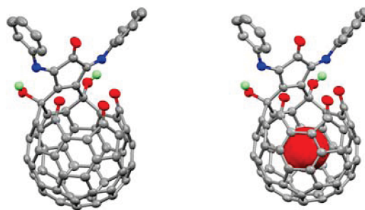
Figure 1. Molecular structures of 1a (left) and \text{H}_2\text{O}@\mathbf{1a} (right). The oxygen atom of the encapsulated water molecule was drawn as the spacefill model. For clarity only the hydrogen atoms of the OH groups were shown. Color scheme: gray, C; red, O; blue, N; green, H.
