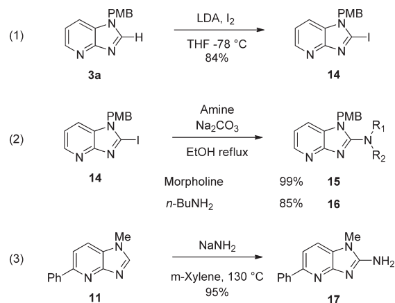
Scheme 3. Product Functionalization
