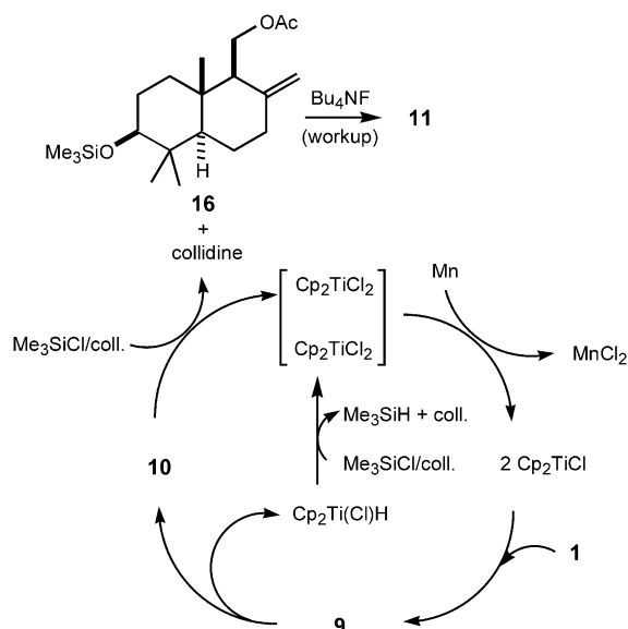
Scheme 2. Hypothetical catalytic cycle for the \text{Ti}^{\text{III}} mediated cyclization of 1 to 11 .
