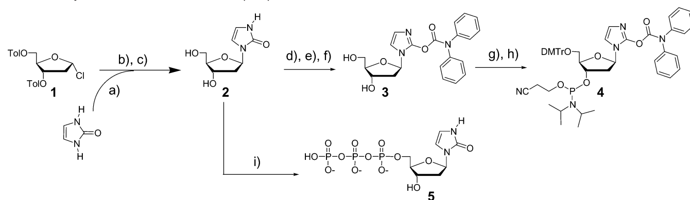
Scheme 1. Synthesis of the Amidite and the Triphosphate of z a
