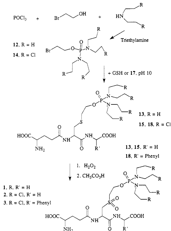
Figure 8. Synthesis of 1, 2, and 3.
