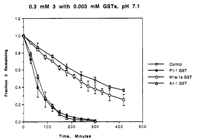
Figure 4. Differential cleavage of 3 by GSTs.
