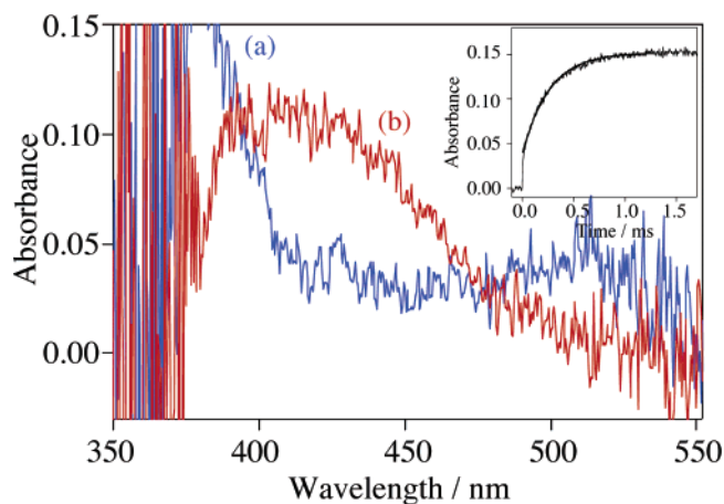
Figure 6. Transient absorption spectra obtained in LFP of U-1 – \text{N}_2 (a) in degassed benzene and (b) in nondegassed benzene with a 308-nm excimer laser recorded 500 \mu\text{s} after the pulse. The inset shows oscillogram traces monitored at 420 nm.
