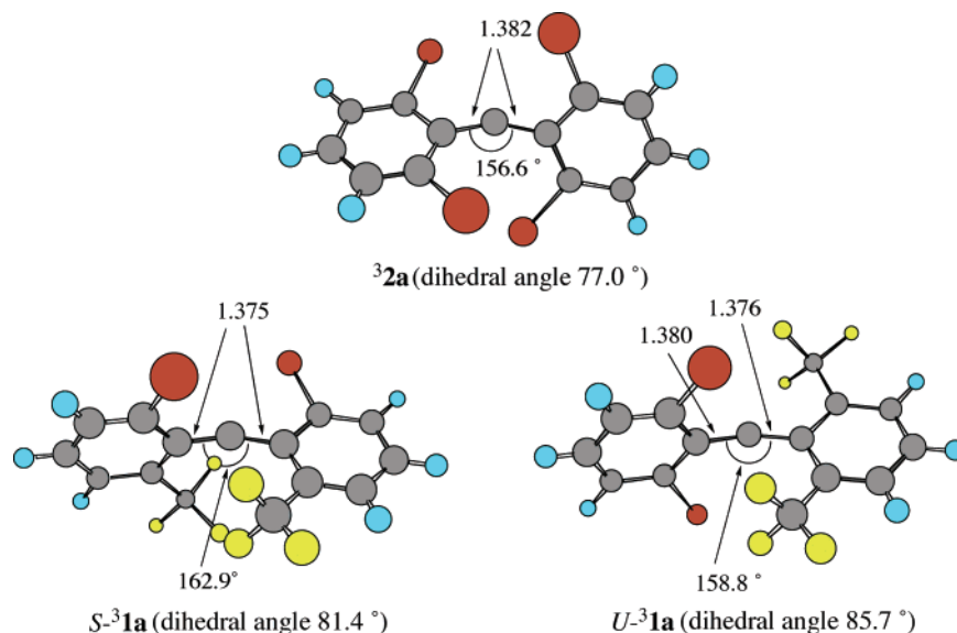
Figure 10. Selected geometrical parameters (distance in Å and angle in deg) for triplet bis(2,6-dibromophenyl)carbene ( ^3\mathbf{2a} ), [2,6-bis(trifluoromethyl)phenyl][2,6-dibromophenyl]carbene ( U\text{-}^3\mathbf{1a} ), and bis(2-bromo-6-trifluoromethylphenyl)carbene ( S\text{-}^3\mathbf{1a} ) at B3LYP/6-31G* level of theory.
