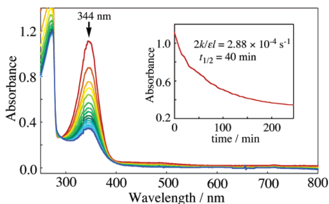
Figure 5. Absorption of transient products formed during irradiation of diazo compound S-1 – \text{N}_2 in degassed benzene at room temperature recorded from immediately after irradiation to 300 min after excitation. The inset shows the time course of the absorption at 344 nm.
