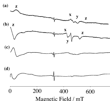
Figure 1. (a) ESR spectrum obtained by irradiation of diazo compound U - 1 -N 2 in 2-methyltetrahydrofuran at 77 K. (b) The same sample measured at 77 K after thawing to 110 K. (c) ESR spectrum obtained by irradiation of diazo compound S - 1 -N 2 in 2-methyltetrahydrofuran at 77 K. (d) The same sample measured at 77 K after thawing to 110 K.
