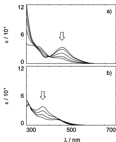
Fig. 8 (a) Changes in the UV-Vis spectrum of rac - 8a (3 mL, 2.71 \times 10^{-6} \text{ mol dm}^{-3} in MeCN containing 0.05 \text{ mol dm}^{-3} \text{ Bu}_4\text{NBF}_4 as a supporting electrolyte) upon constant-current electrochemical reduction (0.1 mA, 5 min intervals). (b) Changes in the UV-Vis spectrum of rac - 8b (3 mL, 6.87 \times 10^{-6} \text{ mol dm}^{-3} in MeCN containing 0.05 \text{ mol dm}^{-3} \text{ Bu}_4\text{NBF}_4 as a supporting electrolyte) upon constant-current electrochemical reduction (0.1 mA, 5 min intervals).
