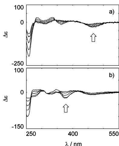
Fig. 9 (a) Changes in the CD spectrum of optically pure ( S,S )- 8a (3 mL, 2.71 \times 10^{-6} \text{ mol dm}^{-3} in MeCN containing 0.05 \text{ mol dm}^{-3} \text{ Bu}_4\text{NBF}_4 as a supporting electrolyte) upon constant-current electrochemical reduction (0.1 mA, 5 min intervals). (b) Changes in the CD spectrum of optically pure ( S,S )- 8b (3 mL, 5.89 \times 10^{-6} \text{ mol dm}^{-3} in MeCN containing 0.05 \text{ mol dm}^{-3} \text{ Bu}_4\text{NBF}_4 as a supporting electrolyte) upon constant-current electrochemical reduction (0.1 mA, 5 min intervals).
