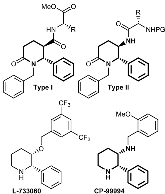
Fig. 1. Substituted piperidinones of types I and II.
