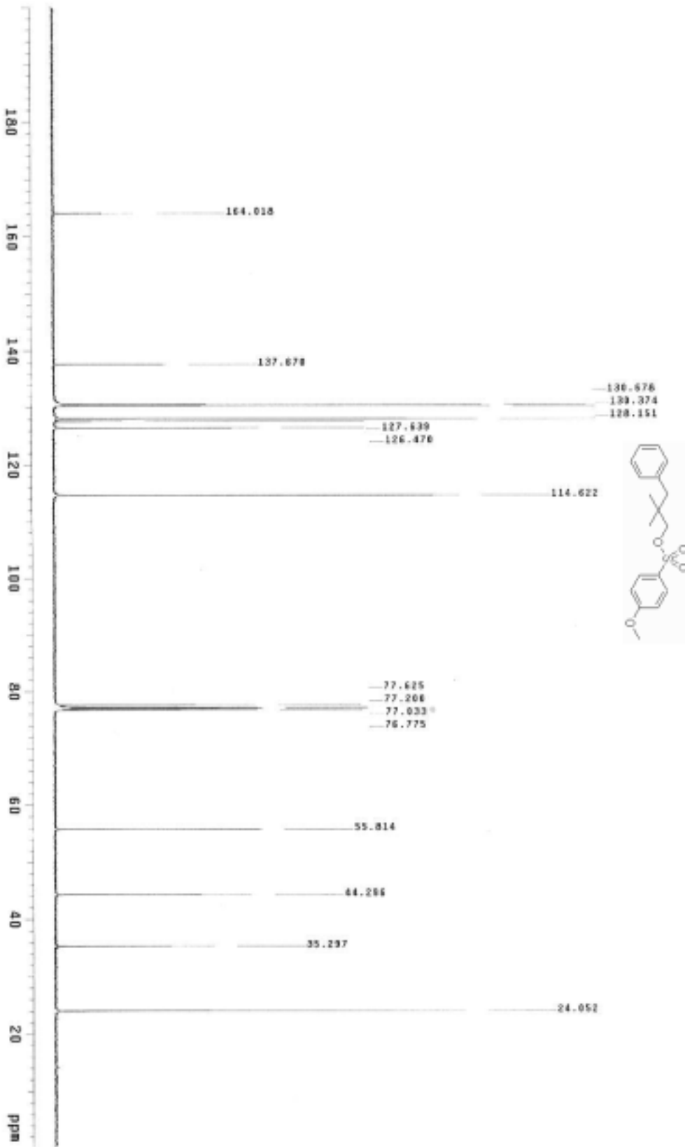
Figure S10. ^{13}\text{C} NMR spectrum of 1e
