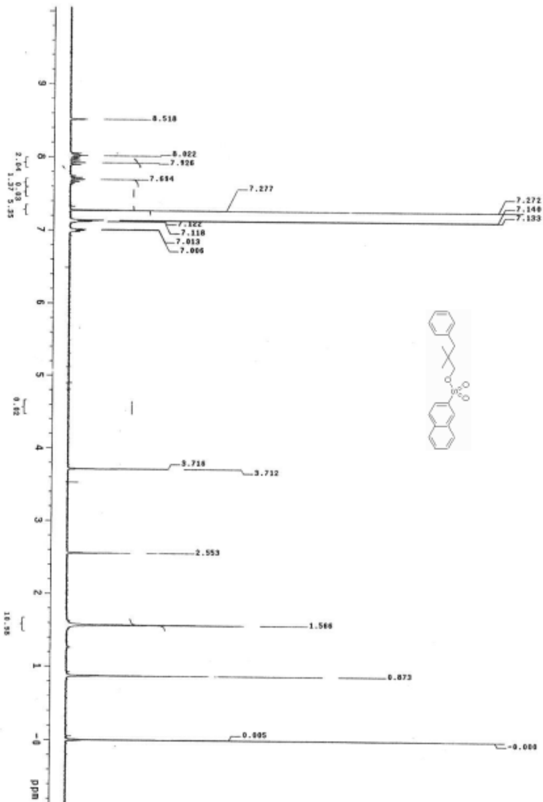
Figure S11. ^1\text{H} NMR spectrum of 1f
