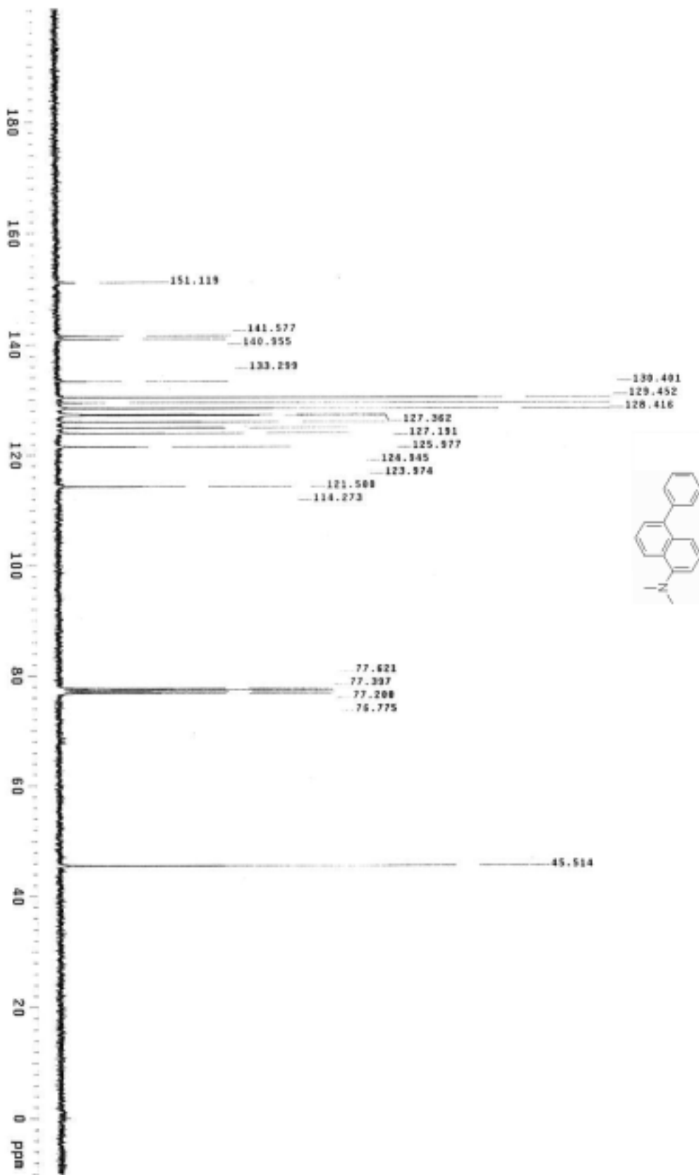
Figure S36. ^{13}\text{C} NMR spectrum of 3r
