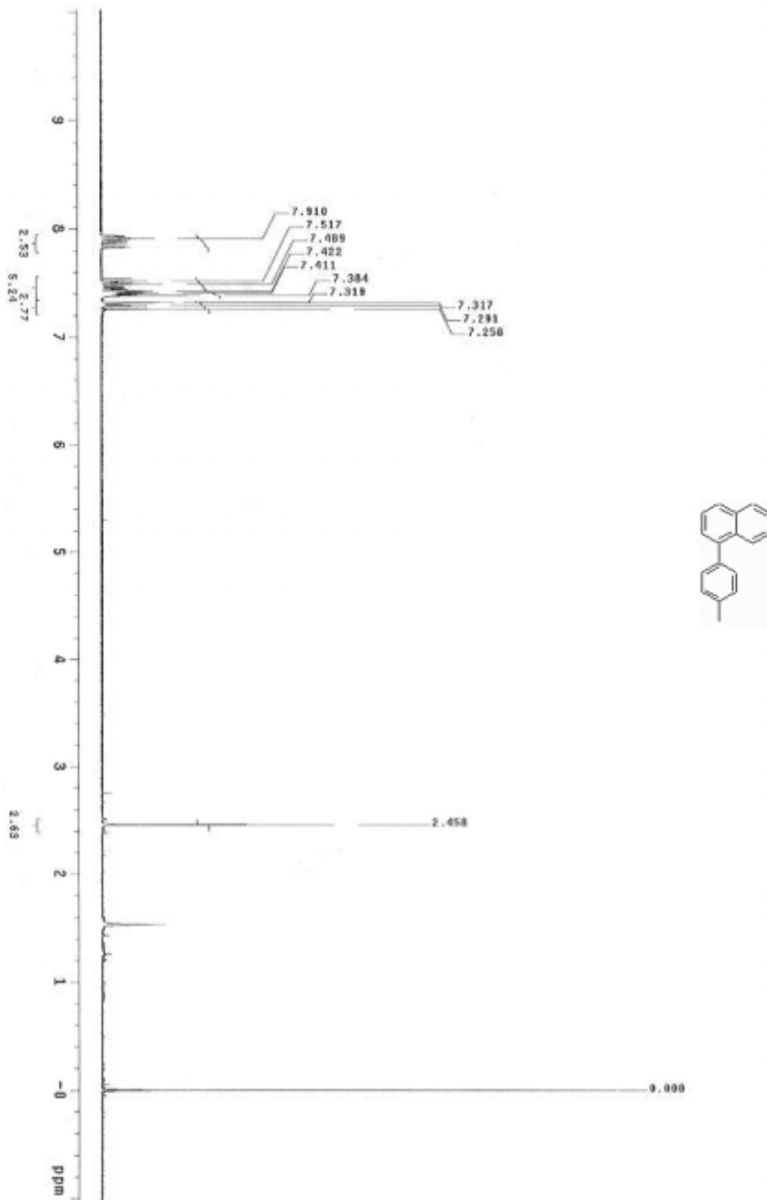
Figure S23. ^1\text{H} NMR spectrum of 3g
