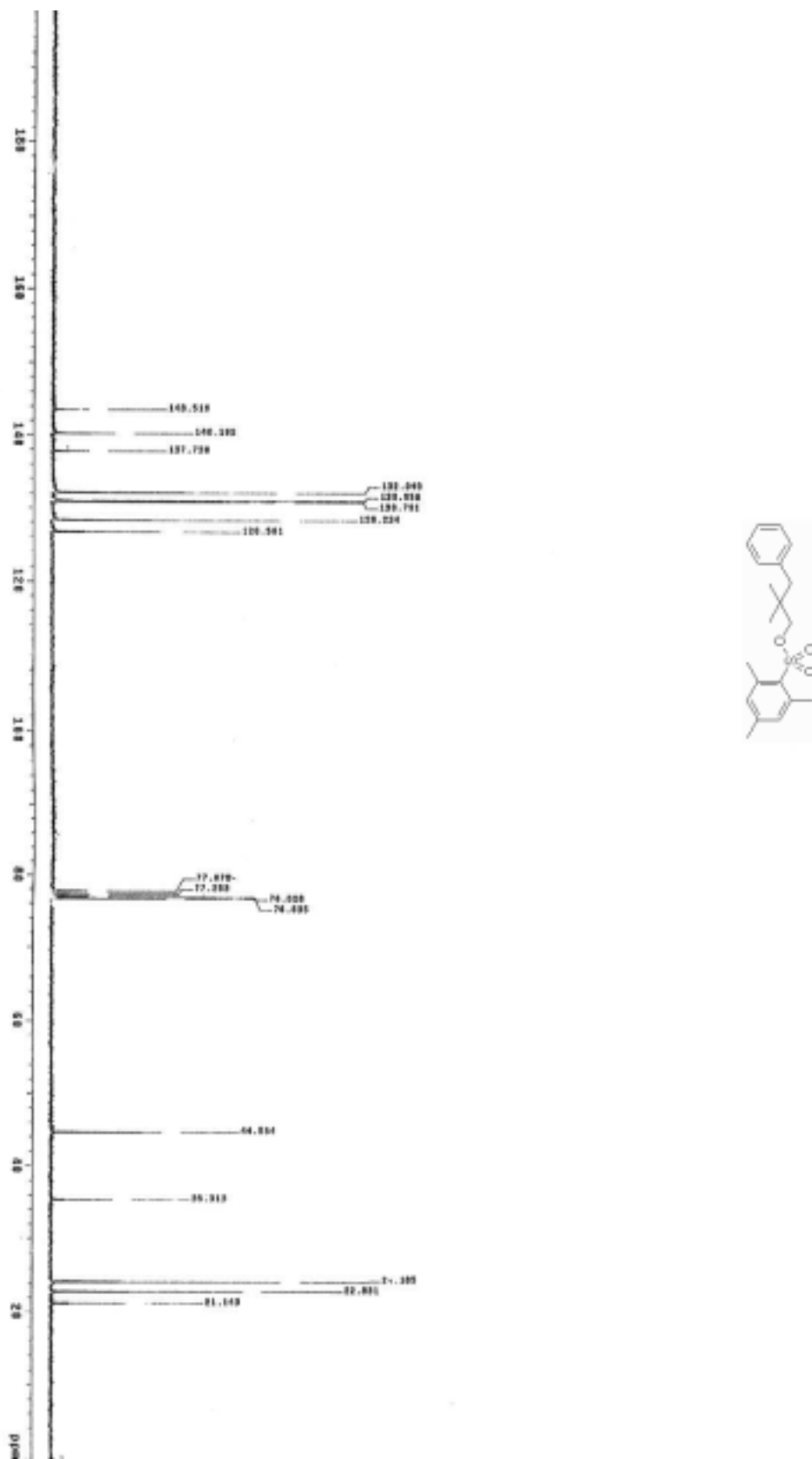
Figure S8. 13 C NMR spectrum of 1d
