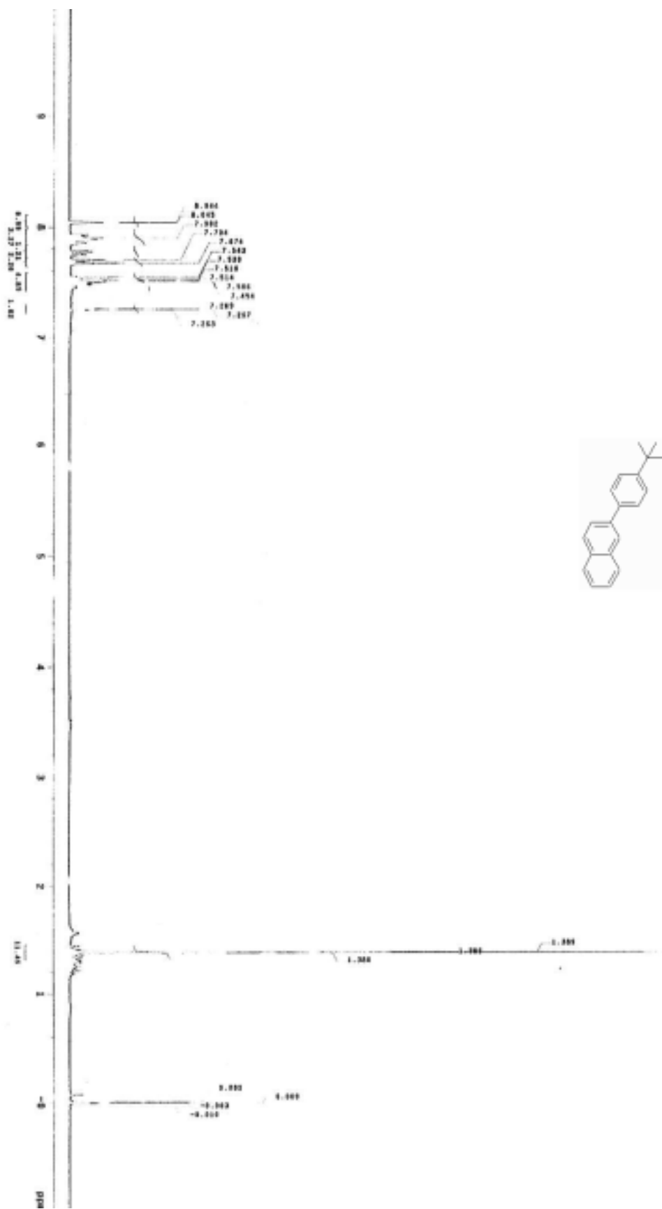
Figure S31. 1 H NMR spectrum of 3p
