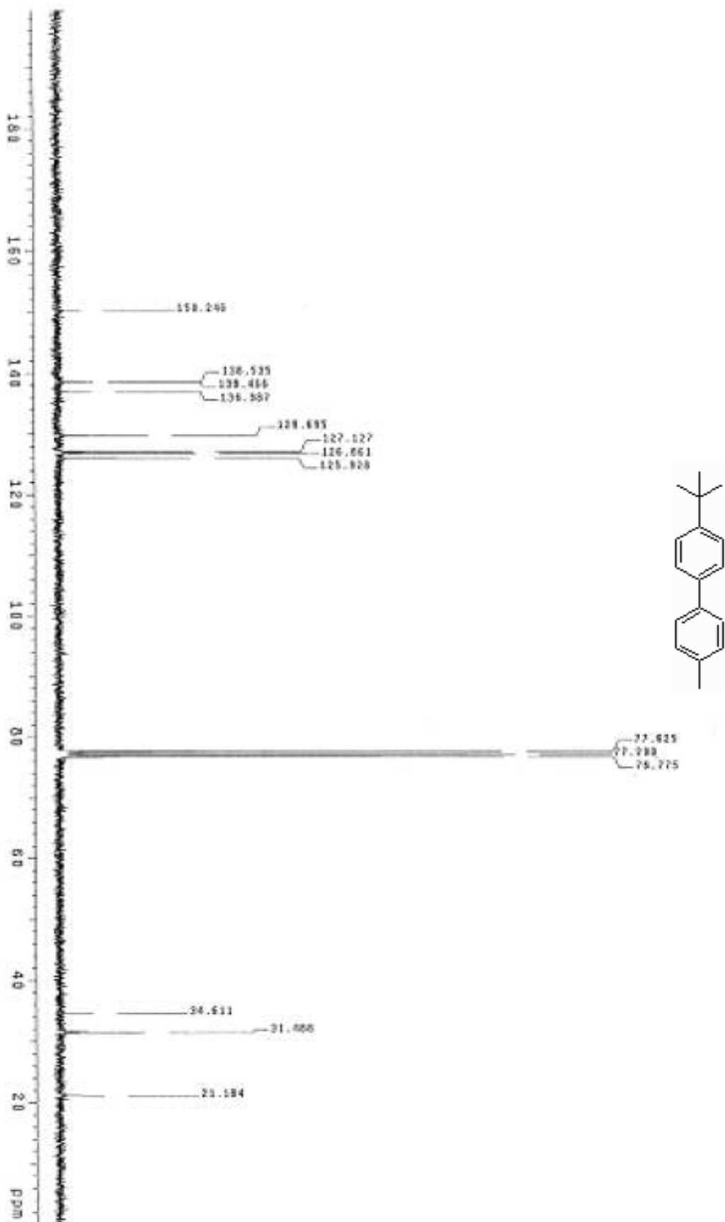
Figure S20. ^{13}\text{C} NMR spectrum of 3b
