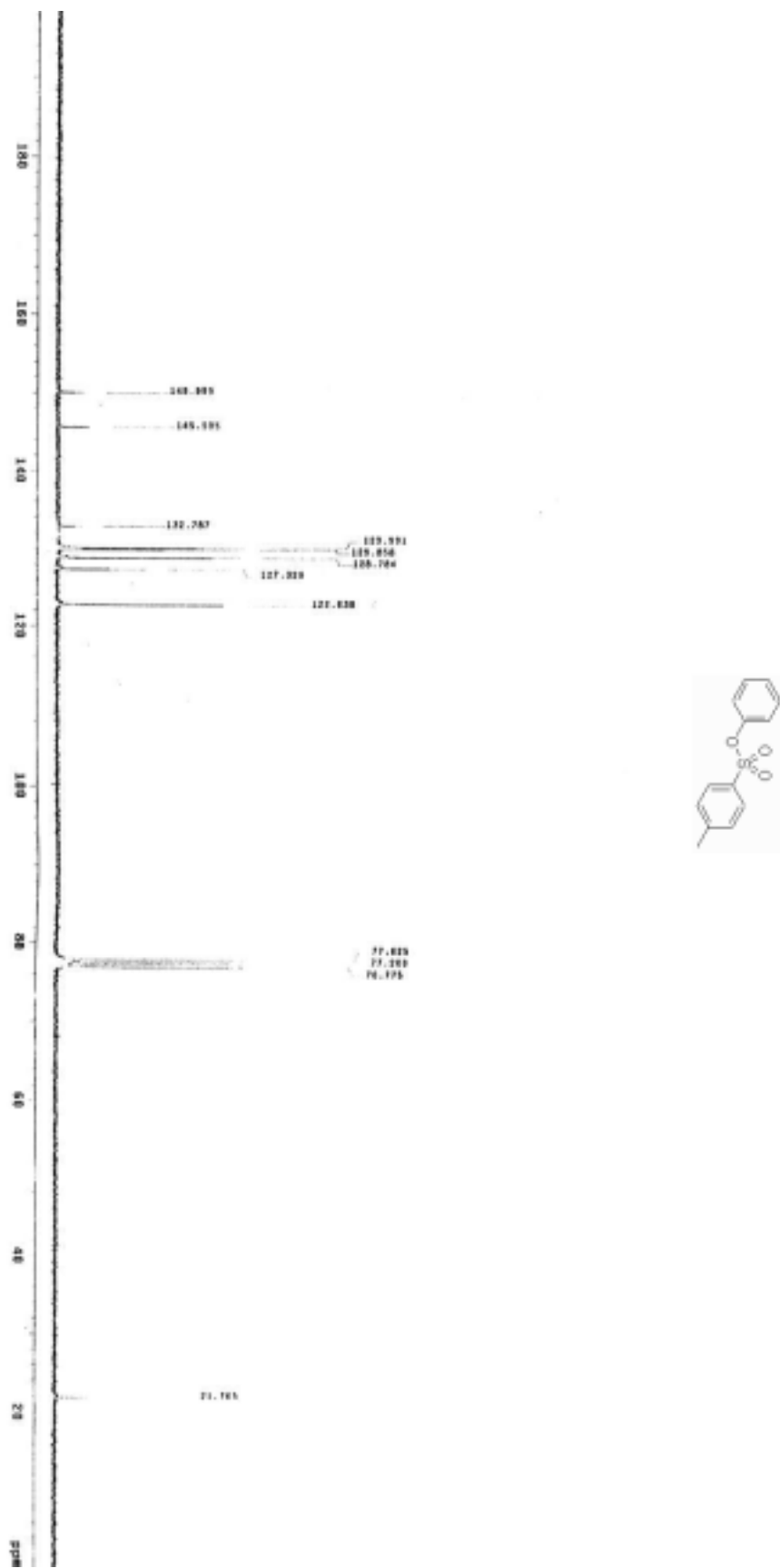
Figure S18. ^{13}\text{C} NMR spectrum of 1i
