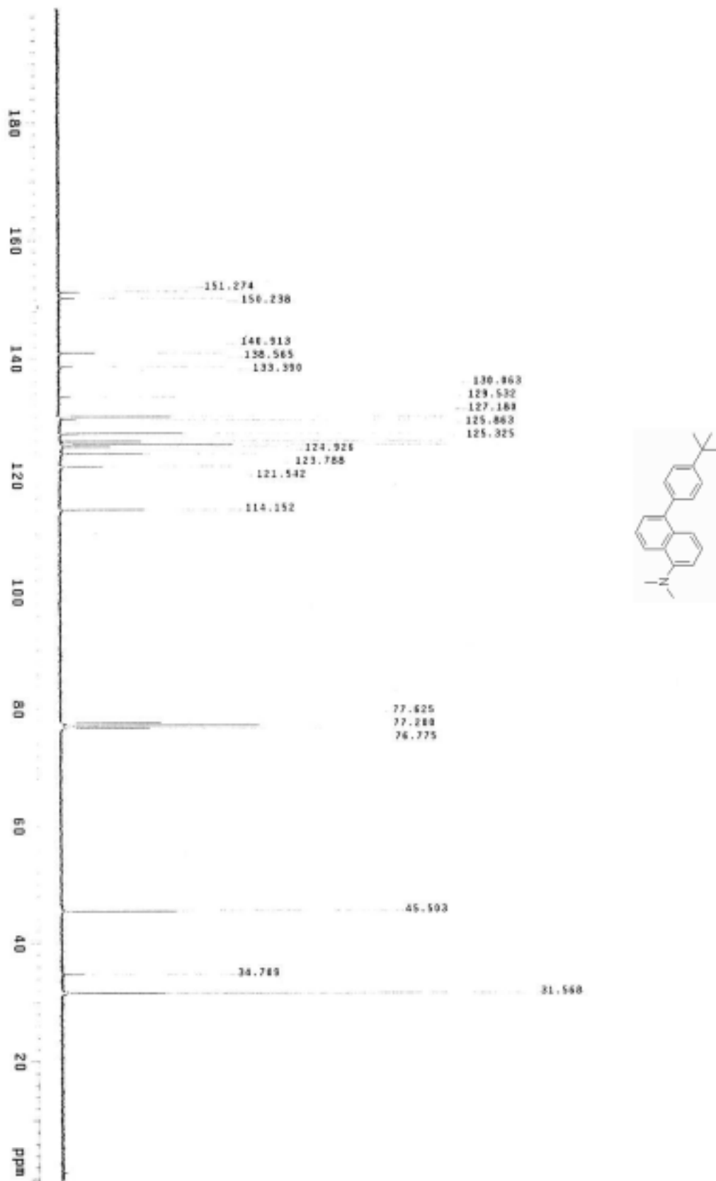
Figure S38. ^{13}\text{C} NMR spectrum of 3s
