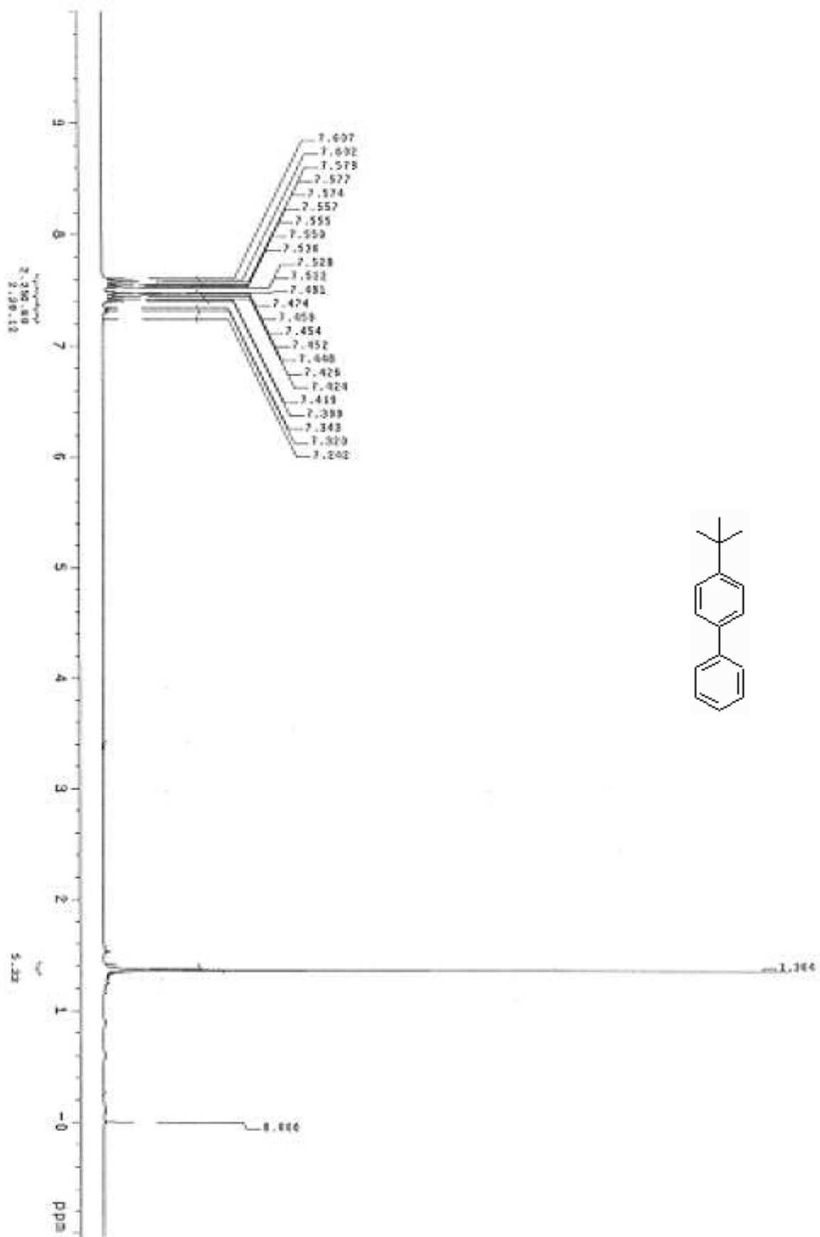
Figure S25. 1 H NMR spectrum of 3i
