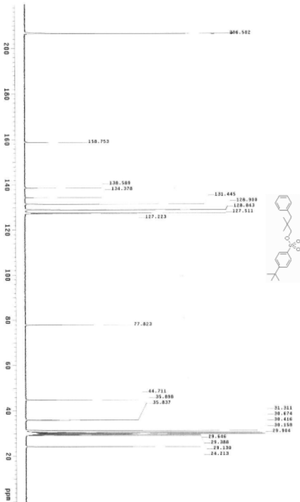
Figure S6. ^{13}\text{C} NMR spectrum of 1c
