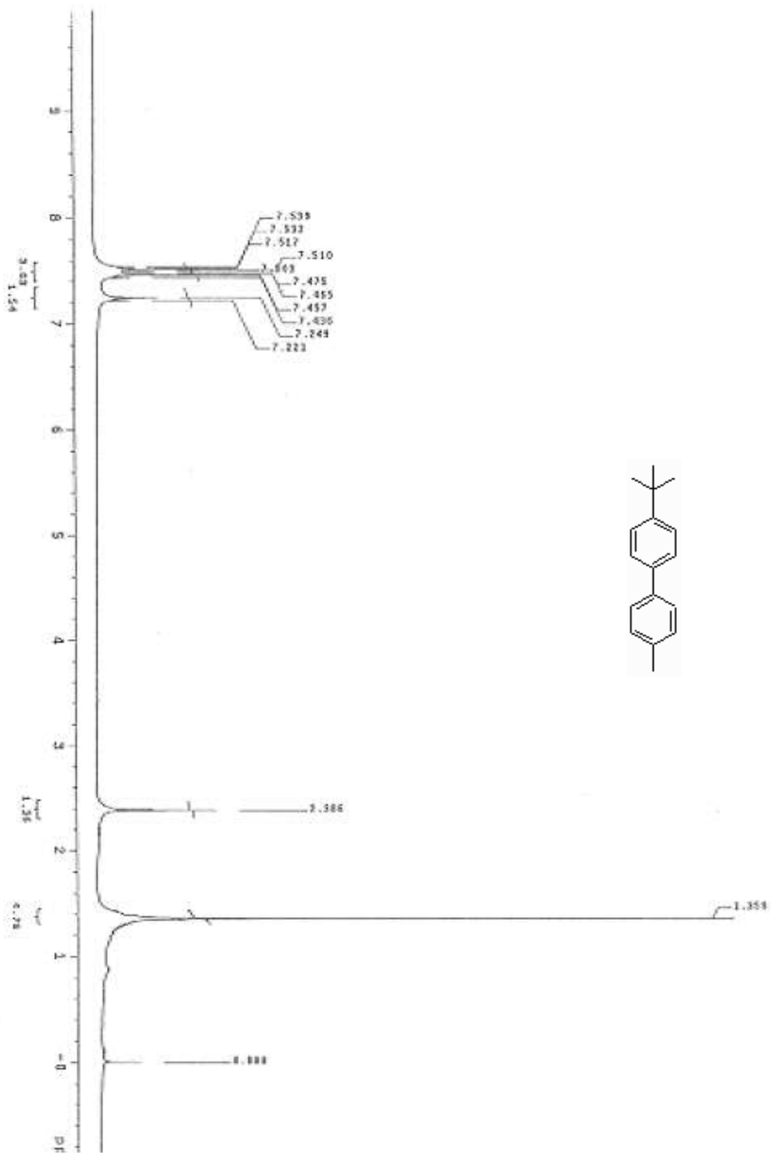
Figure S19. ^1\text{H} NMR spectrum of 3b
