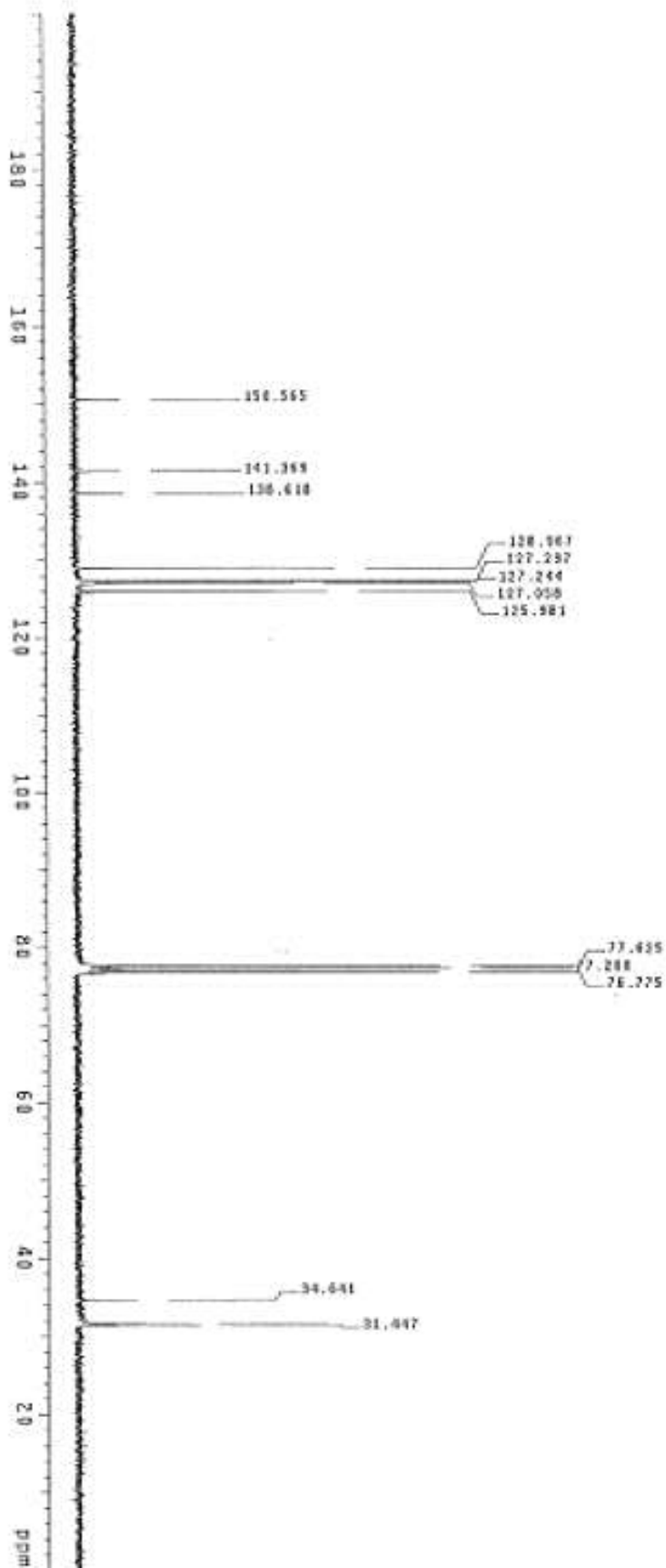
Figure S26. 13 C NMR spectrum of 3i
