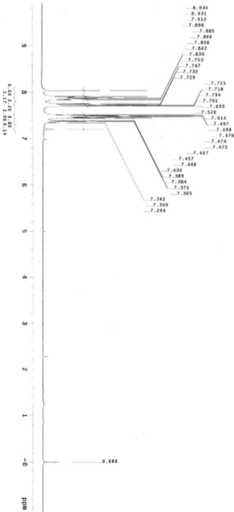
Figure S29. ^1\text{H} NMR spectrum of 3o
