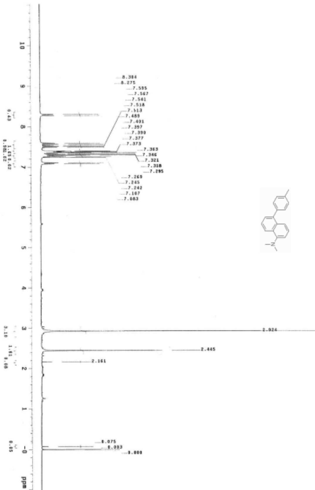
Figure S39. ^1\text{H} NMR spectrum of 3t
