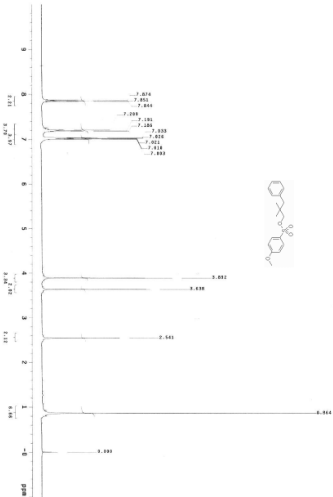
Figure S9. 1 H NMR spectrum of 1e
