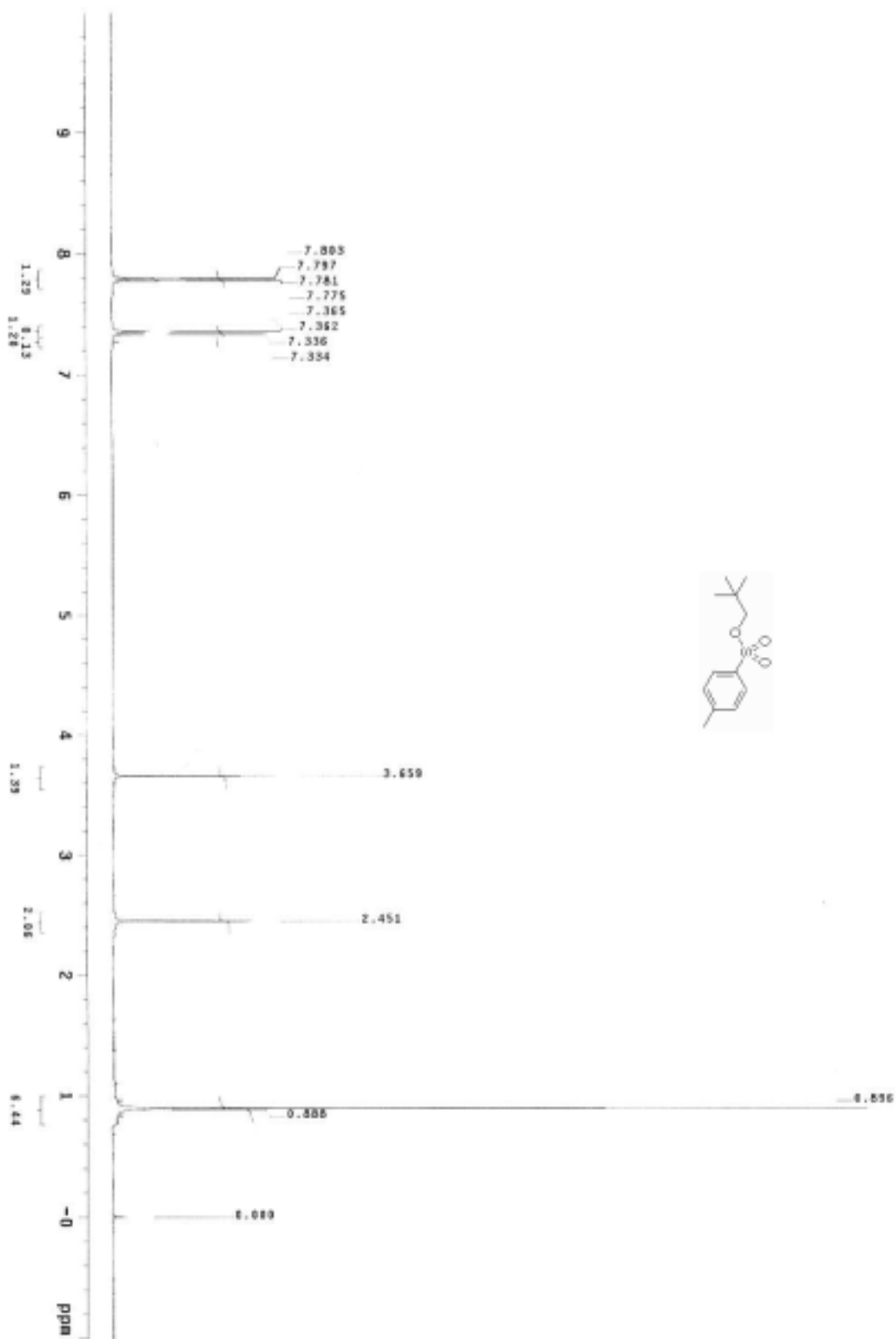
Figure S3. 1 H NMR spectrum of 1b
