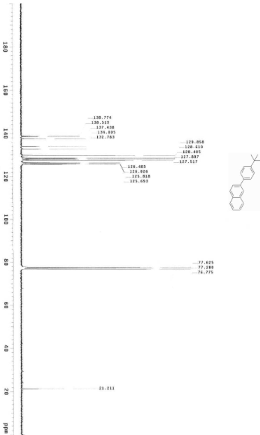
Figure S34. ^{13}\text{C} NMR spectrum of 3q
