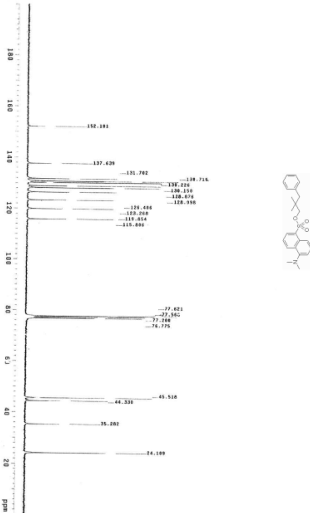
Figure S14. ^{13}\text{C} NMR spectrum of 1g
