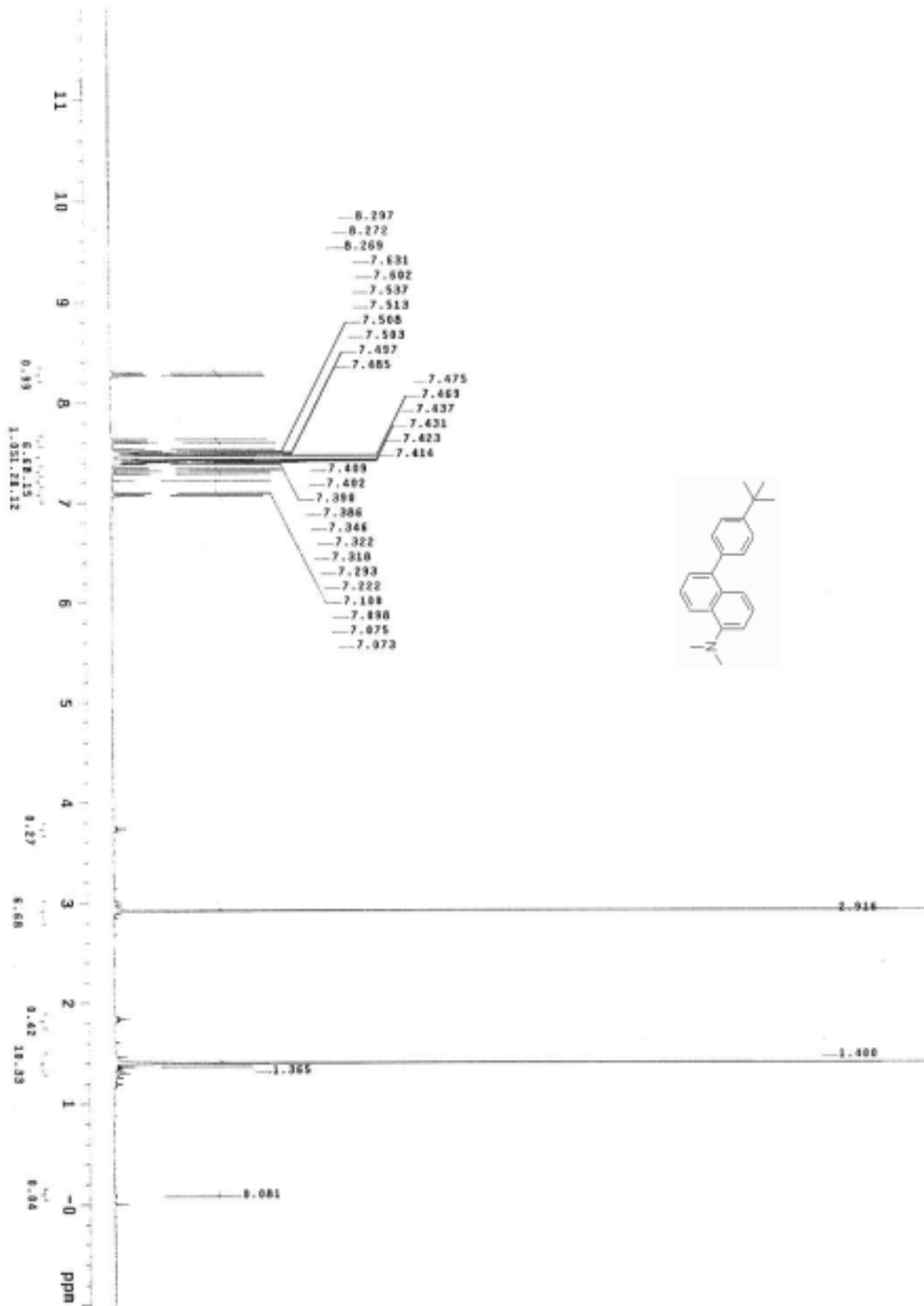
Figure S37. ^1\text{H} NMR spectrum of 3s
