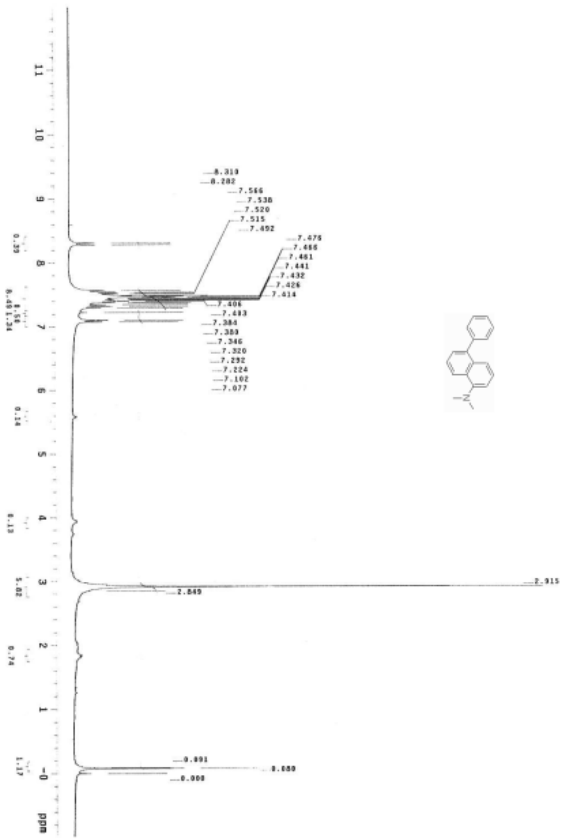
Figure S35. 1 H NMR spectrum of 3r
