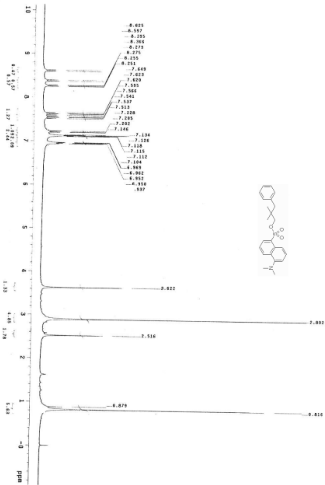
Figure S13. 1 H NMR spectrum of 1g
