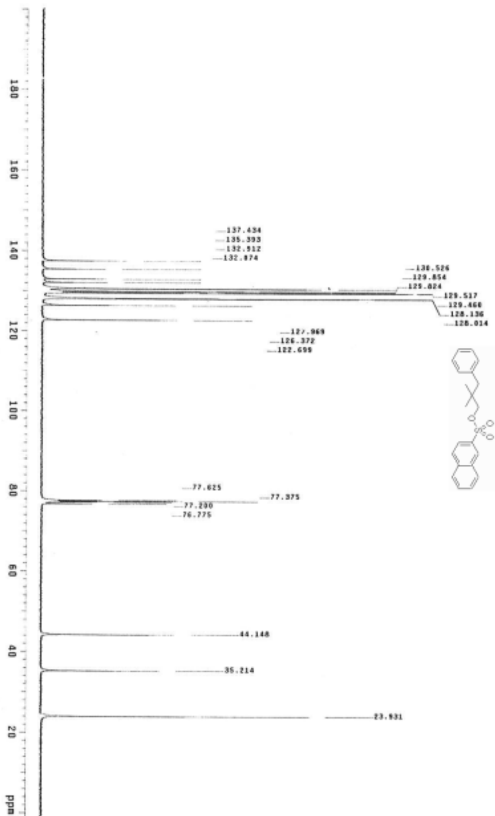
Figure S12. ^{13}\text{C} NMR spectrum of 1f
