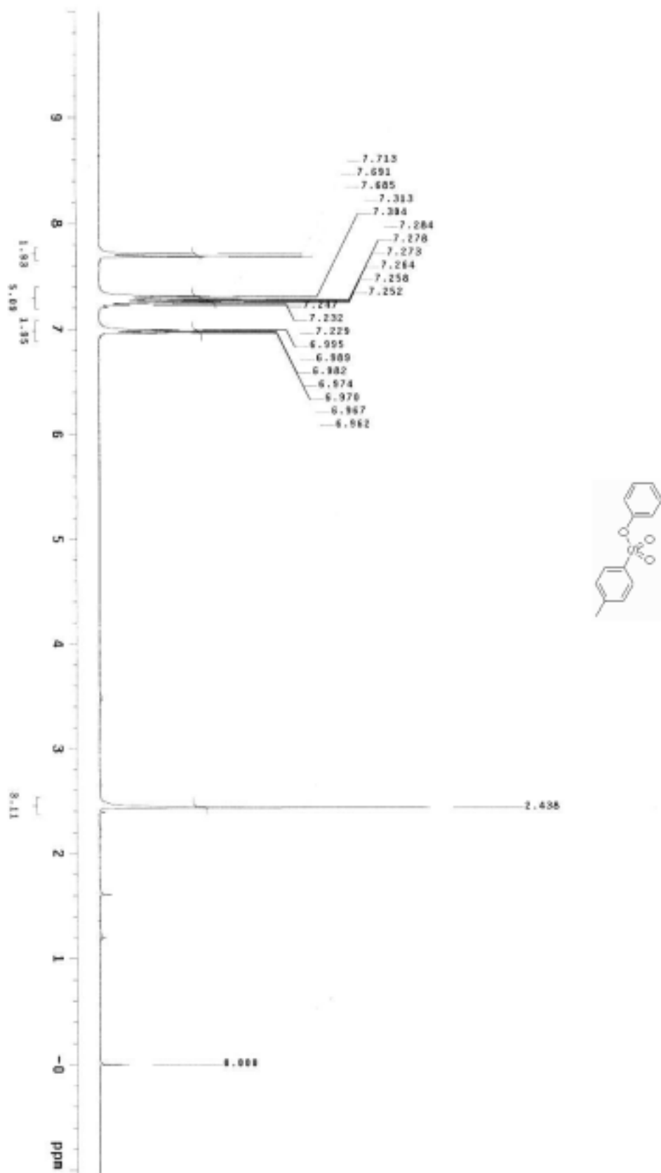
Figure S17. ^1\text{H} NMR spectrum of 1i
