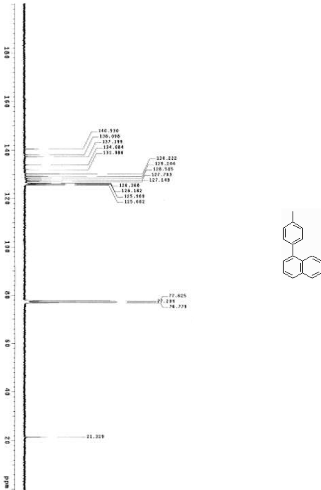
Figure S24. ^{13}\text{C} NMR spectrum of 3g
