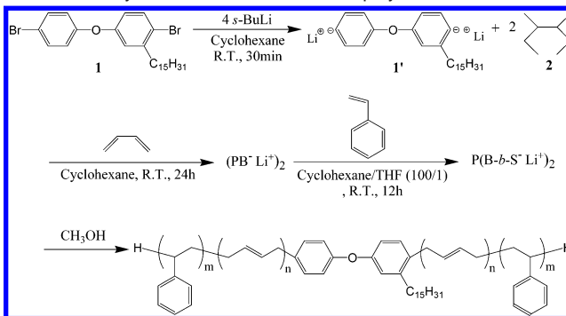
Scheme 1. Synthesis of SBS Triblock Copolymers
