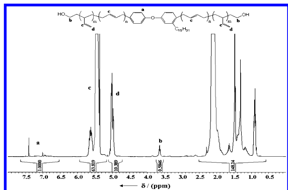
Figure 1. ^1\text{H} NMR spectrum ( \text{CD}_2\text{Cl}_2 , 400 MHz) of a \alpha,\omega -dihydroxy-terminated polybutadiene.
