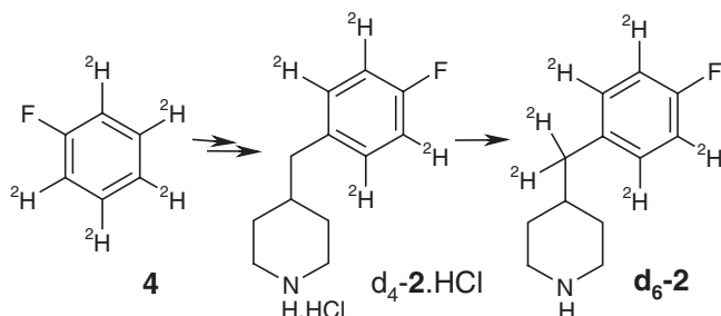
Scheme 3. Preparation of the d_4 -, d_2 -2 and d_6 -2 isotopomers (i: \text{Br}_2 , \text{FeCl}_3 , \text{CH}_2\text{Cl}_2 ; ii: \text{Mg} , THF then pyridine-4-aldehyde; iii: \text{H}_2 , \text{Pd/C} \text{CH}_3\text{OH} ; iv: ^2\text{H}_2 , \text{Pd/C} , \text{C}^2\text{H}_3\text{O}^2\text{H} , ^2\text{HCl} )
