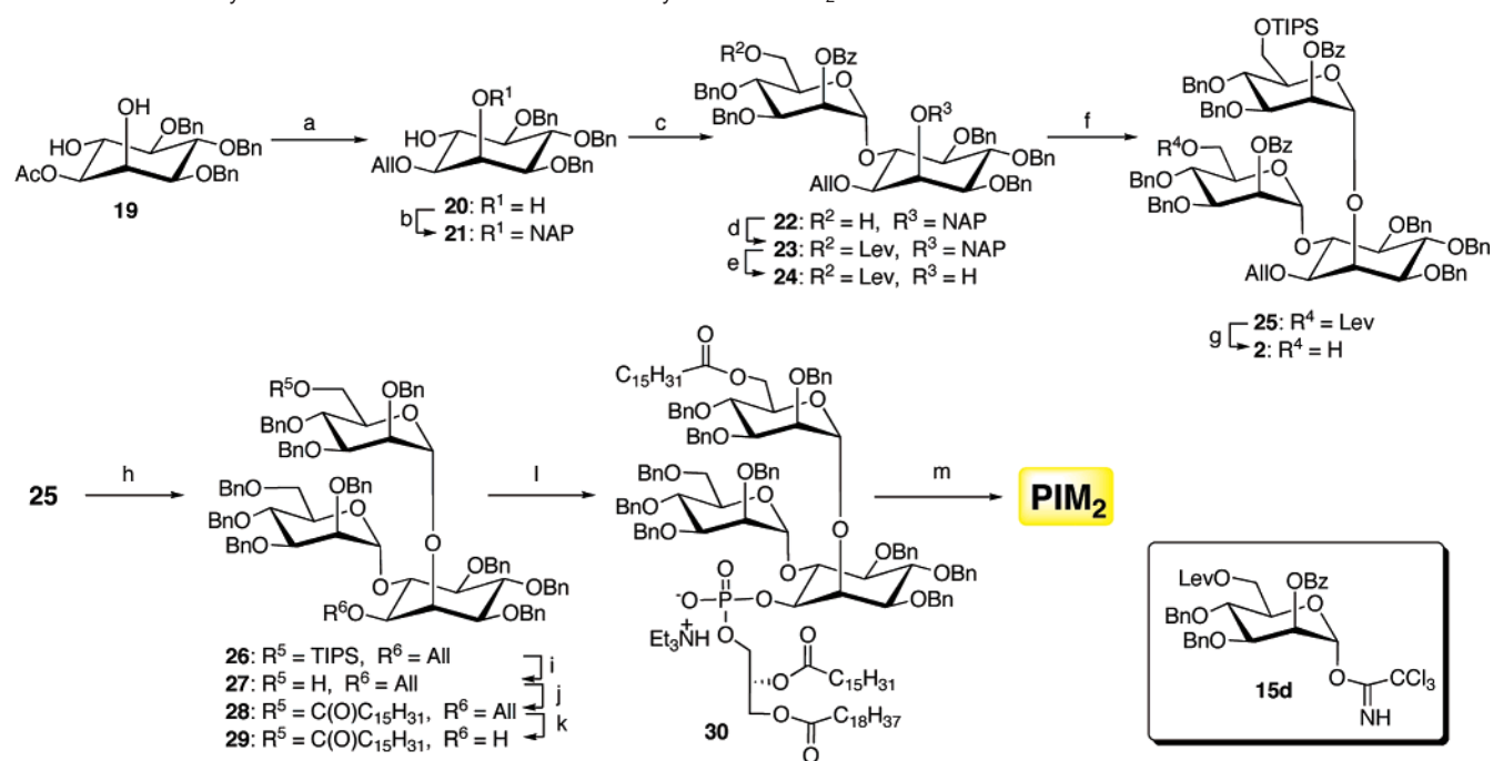
Scheme 3. Assembly of Inositol Dimannnoside 2 and Total Synthesis of PIM 2 a
