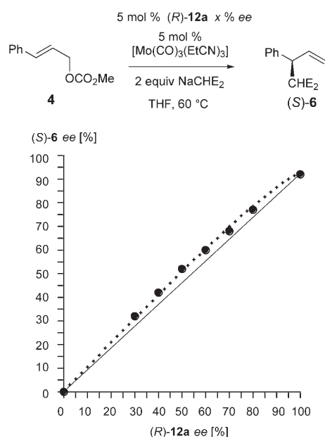
Figure 1. Non-linear relationship between the enantiomeric excess of ligand ( R )- 12a and branched product ( S )- 6 obtained on asymmetric Mo-catalyzed allylic alkylation of 4 . ●: data points from experiments; ----: linear correlation; +: calculated relationship based on the Kagan “reservoir model” for ML_2 with g=0 and K=0.06 . [39a]
