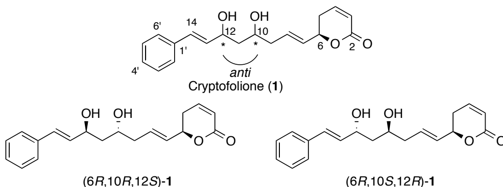
Figure 1. Two possible stereoisomers, (6 R ,10 R ,12 S )- 1 and (6 R ,10 S ,12 S )- 1 , for cryptofolione.
