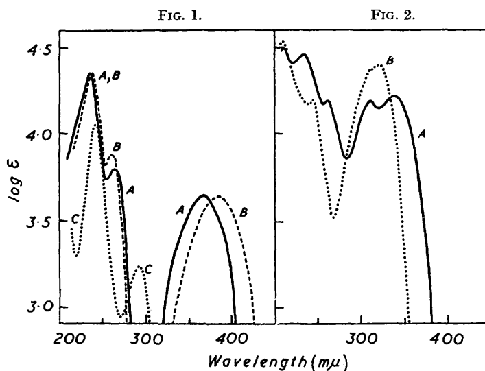
FIG. 1. Ultraviolet spectra of ethanolic solutions of (A) 4:5:6:7-tetrahydro-1-methyl-4-oxo-2:3-benzazepine (I; R = Me), (B) 1:2:3:4-tetrahydro-1-methyl-4-oxoquinoline (II), and (C) \beta -tetralone (see also Biquard 12 ). Curves (A) and (B) have minima at 294 m \mu (log \epsilon 2.556) and 288 m \mu (log \epsilon 1.740) respectively, which are not shown.
