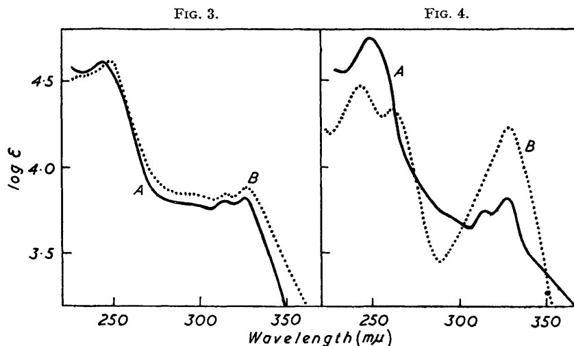
FIG. 3. Ultraviolet spectra of 6:7-dihydro-1-methyl-2:3-benzoquinolino(2':3'-4:5)azepine-4'-carboxylic acid (XV; \text{R} = \text{CO}_2\text{H} ), (A) in 0.1\text{N-NaOH} , (B) in ethanol.
