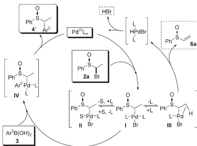
Scheme 4. Catalytic cycle of the palladium-catalyzed reaction of (±)- 2a with boronic acids.
