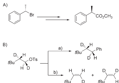
Scheme 1. Palladium-catalyzed reactions at stereogenic carbon centers. A) 1) \text{Pd}(\text{PPh}_3)_4/\text{CO} ; 2) \text{Br}_2 ; 3) \text{CH}_3\text{OH} ; B) \text{Pd}/\text{PtBu}_2\text{Me} and a) 9-BBN-Ph (BBN=9-borabicyclo[3.3.1]nonane) or b) dioxane, 70 °C.
