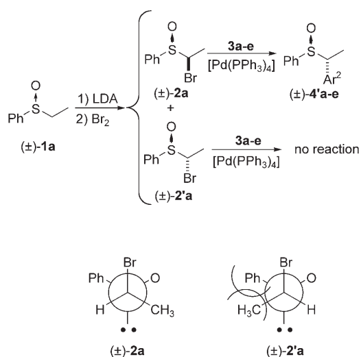
Scheme 5. Palladium-catalyzed cross-coupling reaction of (±)- 2'a and (±)- 2a .
