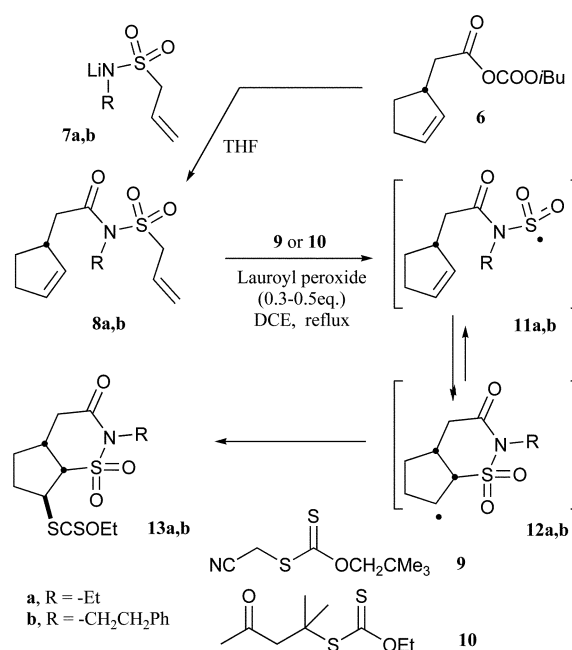
Scheme 2 Formation of cyclic N -sulfonylamides.
