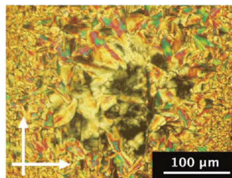
Figure 3. Polarized optical micrograph of the tripodal pyridinium salt Py1 at 235 °C in the Col phase. Arrows indicate the directions of polarizer and analyzer axes.
