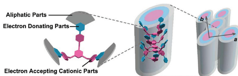
Figure 4. A schematic representation of the self-assembled columnar structure of tripodal salts. \text{PF}_6 anions are omitted for clarity.
