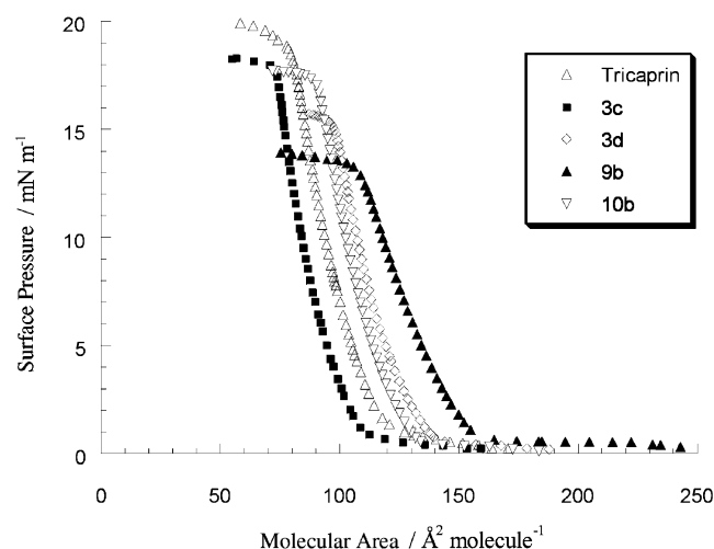
Figure 2. Force/area curves of the tricaprin analogues. The aqueous subphase was composed of Tris/HCl (10 mM, pH 8.0), NaCl (100 mM), CaCl 2 (21 mM), and EDTA (1 mM). The continuous compression experiments were performed in the rectangular reservoir of the zero-order trough.
