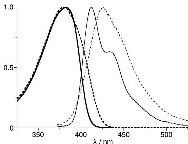
Figure 7. Normalised absorption spectra (bold) and emission spectra (plain) of 2C\beta -CD (—) and 2 (----) in aqueous solution (both \bar{n}_{\text{Nom}} = 10 ; 1.66 mM LiOH, 2.11 mM \text{Li}_2\text{CO}_3 aqueous buffer, pH 9; emission spectra with excitation at 361 nm).
