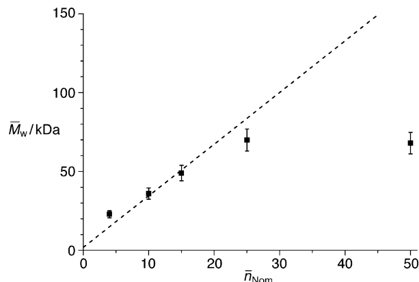
Figure 6. Plot of \bar{M}_w(\text{AUC}) versus \bar{n}_{\text{Nom}} for 1Cβ-CD . The straight line shows the ideal behaviour in the absence of accidental termination or fractionation during purification (assuming a threading ratio of \bar{y} = 1.1 ).
