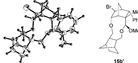
Scheme 8. X-ray crystal structure of 15b' .
