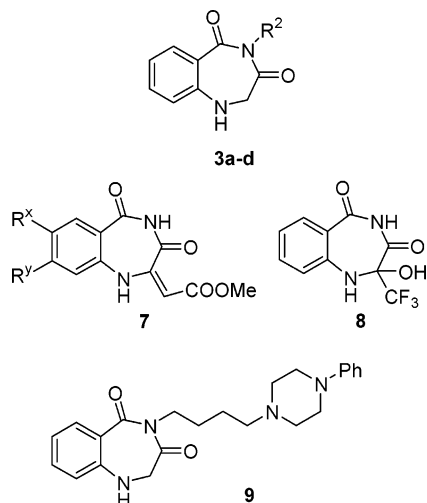
FIGURE 1. Compounds 3a ( R^2 = \text{Et} ) 5 and 3b–d ( b , R^2 = \text{Ph} ; c , R^2 = \text{Bn} ; d , R^2 = p\text{-toluyl} ), 6 7 ( R^x and R^y combinations of H, Me, OMe, F, Cl, Br, and I), 7,8 and compounds similar to 9 . 9,10 appear in the literature.
