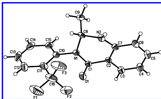
FIGURE 2. ORTEP diagram of 6f .
