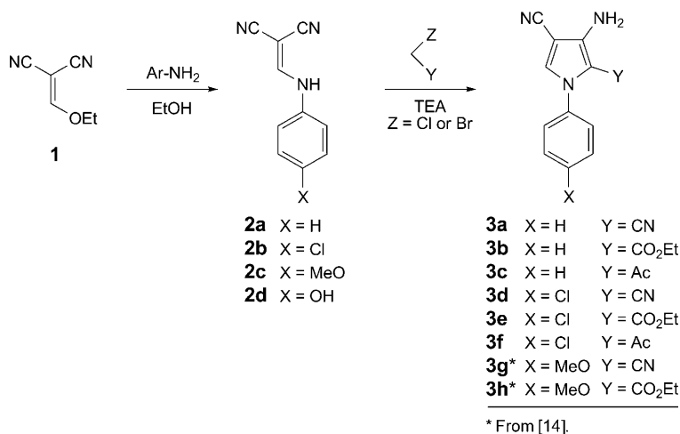
Scheme 1. Synthesis and Structure of Compounds 3
