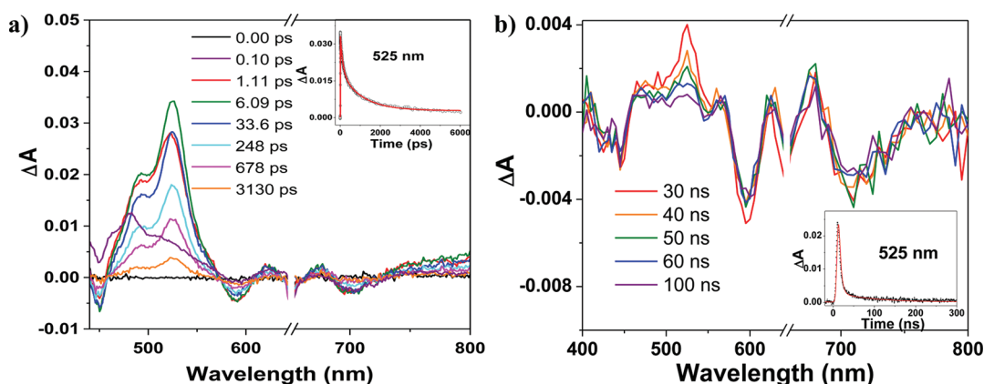
Figure 7. (a) Femtosecond and (b) nanosecond transient absorption spectra of neat TIPS-Pn films ( \lambda_{\text{ex}} = 650 nm). The insets show the transient decay kinetics at 525 nm.
