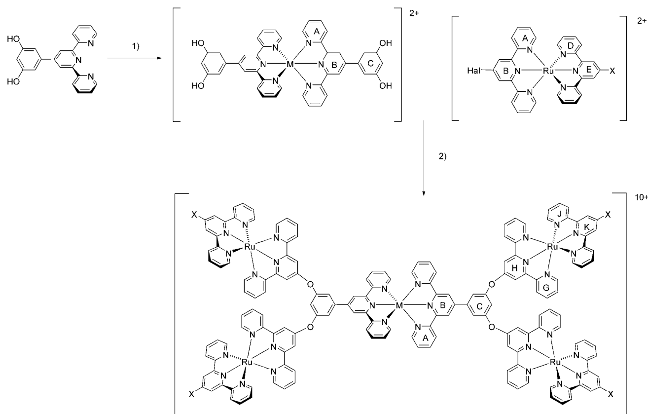
Scheme 4. Synthesis of the dendritic pentanuclear complexes showing the ring-labelling scheme adopted. 1) \text{RuCl}_3 \cdot 3\text{H}_2\text{O} or \text{K}_2[\text{OsCl}_6] , ethane-1,2-diol, N -ethylmorpholine, microwave; 2) \text{K}_2\text{CO}_3 , MeCN; \text{M} = \text{Os} or \text{Ru} , \text{X} = \text{H} (tpy) or 2-thienyl ( 5 ). In the case of the complexes with 5 , the thienyl ring is labelled L.
