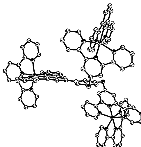
Figure 1. MMFF (Spartan '04) minimised structure of the trinuclear V-shaped complex [(\text{tpy})\text{Ru}(\mathbf{6})\{\text{Ru}(\text{tpy})\}_2] showing the expected conformation of the ether-linked moieties; the \text{Ru}_{\text{central}}\cdots\text{Ru}_{\text{outer}} and \text{Ru}_{\text{outer}}\cdots\text{Ru}_{\text{outer}} distances are in the ranges 12.3–12.6 Å and 14.0–14.2 Å, respectively. Hydrogen atoms have been omitted for clarity.
