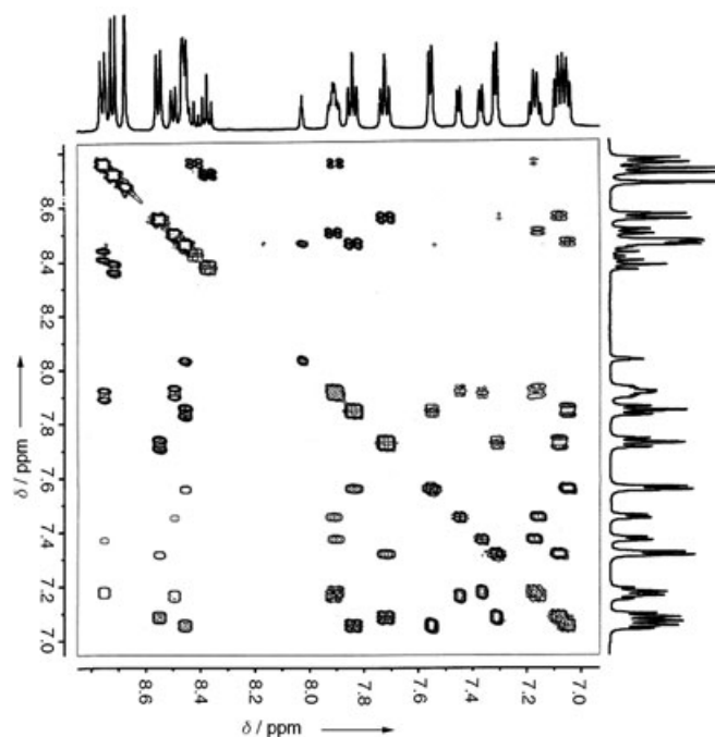
Figure 2. 500 MHz COSY 90 spectrum (room temperature) of a solution of [(\text{tpy})\text{Ru}(\mathbf{6})\{\text{Ru}(\text{tpy})\}_2][\text{PF}_6]_6 in \text{CD}_3\text{CN} .
