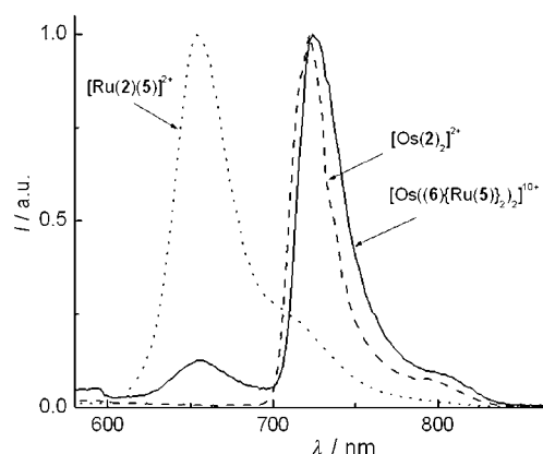
Figure 4. Normalised luminescence spectra at 77 K for [\text{Os}(\text{6})(\text{Ru}(\text{5}))_2]^{10+} (—), [\text{Os}(\text{2})_2]^{2+} (---) and [\text{Ru}(\text{2})(\text{5})]^{2+} (.....); \lambda_{\text{exc}} = 480 \text{ nm} in all cases.
