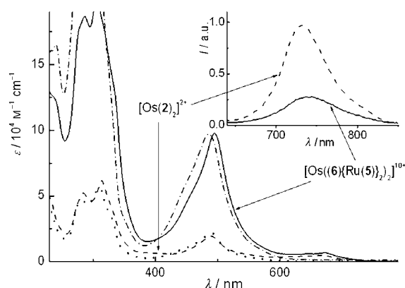
Figure 3. The ground-state absorption spectra of [\text{Os}(\text{6})(\text{Ru}(\text{5}))_2]^{10+} (—), [\text{Os}(\text{2})_2]^{2+} (---), [\text{Ru}(\text{2})(\text{5})]^{2+} (.....) and [\text{Ru}(\text{6})(\text{Ru}(\text{tpy}))_2]^{10+} (-.-.-). The inset shows the room temperature luminescence spectra of [\text{Os}(\text{6})(\text{Ru}(\text{5}))_2]^{10+} (—) and [\text{Os}(\text{2})_2]^{2+} (---), as obtained from isoabsorbing solutions at \lambda_{\text{exc}} = 480 \text{ nm} .
