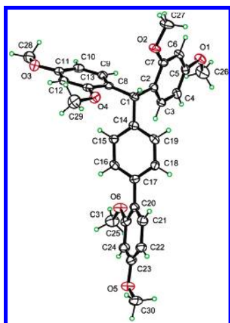
FIGURE 2. X-ray structure for 19 .
