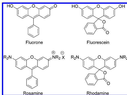
FIGURE 1. Structures of some common xanthene dyes.
