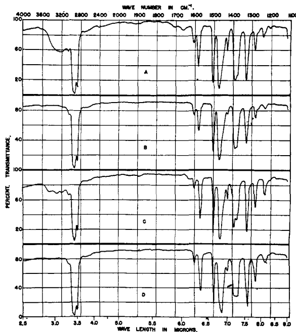
Fig. 2.—Infrared spectra with \text{CaF}_2 prism: A, magnesium 8-quinolinolate dihydrate; B, magnesium 8-quinolinolate; C, bismuth 8-quinolinolate monohydrate; D, bismuth 8-quinolinolate.
