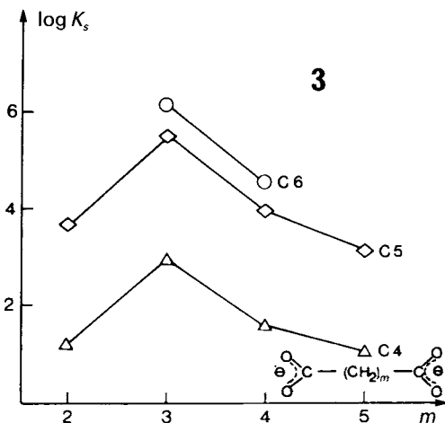
Fig. 4. Graphical representation of the stability constants \log K_s of the complexes formed by the polyammonium macrocycle 3 with the dicarboxylates ^{\ominus}O_2C-(CH_2)_m-CO_2^{\ominus} as a function of chain length m . C4, C5 and C6 correspond to the (3, A^{2-}, nH^+) species with n = 4, 5 , and 6 . See also Table 2.
