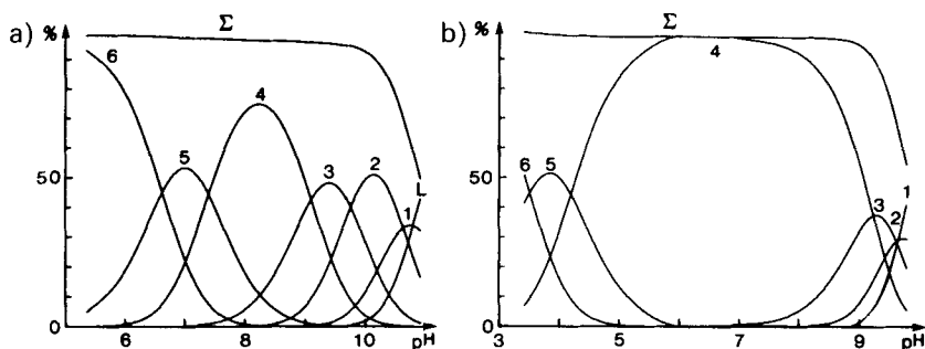
Fig. 1. Distribution curves of the unprotonated and protonated forms of the macrocyclic polyamines as a function of pH; a) compound 1, b) compound 3. L: unprotonated species; the numbers 1–6 refer to the successive protonated species bearing 1–6 protons; \Sigma : summation over all the protonated species. In the case of 3, the unprotonated macrocycle L precipitates and is not represented; \Sigma does not contain LH + .
