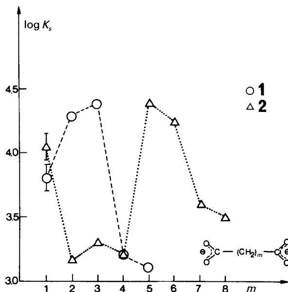
Fig. 3. Graphical representation of the stability constants \log K_s of the complexes formed by the polyammonium macrocycles 1 \cdot 6H^+ ( \circ ) and 2 \cdot 6H^+ ( \triangle ) with the dicarboxylates ^{\ominus}O_2C-(CH_2)_m-CO_2^{\ominus} as a function of chain length m . See also Table 2 and text.
