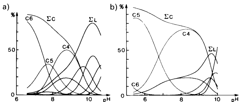
Fig. 2. Distribution curves for the species present in the medium as a function of pH in two cases; a) macrocyclic polyamine 1 , and b) macrocyclic polyamine 3 in presence of glutarate ^{-}\text{O}_2\text{C}-(\text{CH}_2)_3-\text{CO}_2^{-} . C4, C5, C6: complexes (\text{L}, \text{A}^{2-}, n\text{H}^+) with n = 4, 5, 6 . \Sigma \text{C} : summation over all complexes. \Sigma \text{L} : summation over all uncomplexed ligand species (except unprotonated and monoprotonated for 3 ).
