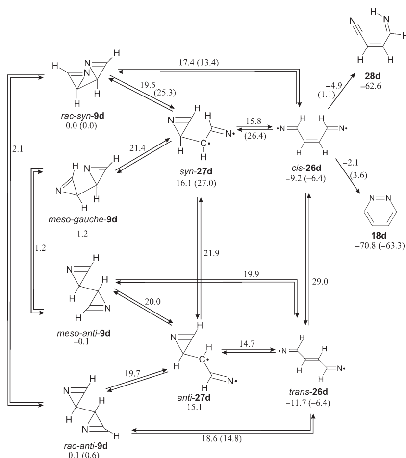
Figure 2. Reactions of the parent bi-2 H -azirin-2-yls 9d that are triggered by C–N bond breaking: Energies at UB3LYP/6-31+G* (ZPVE corrected) relative to rac-syn-9d are given in kcal mol -1 . Relative energies of transition states are given at the corresponding arrows; relative energies (ZPVE-corrected), calculated at the MR-MP2/TZV(2df,2p) level, are given in parentheses.
