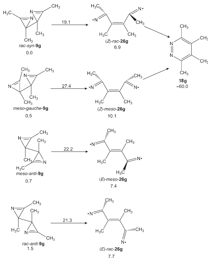
Figure 4. Reactions of tetramethyl-bi-2 H -azirin-2-yls 9g : Energies at UB3LYP/6-31 + G* level (ZPVE-corrected) relative to tetramethylbiazirinyl rac - syn - 9g are given in kcal mol -1 . Energies of transition states are given above the corresponding arrows.
