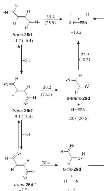
Figure 3. Fragmentation pathways for the E diradical trans - 26d : Energies at UB3LYP/6-31+G* level (ZPVE corrected) in kcalmol -1 are relative to bisaziriny rac - syn - 9d . Energies of transition states are given at the corresponding reaction arrows; relative energies (ZPVE-corrected), calculated at the MR-MP2/TZV(2df,2p) level, are given in parentheses.
