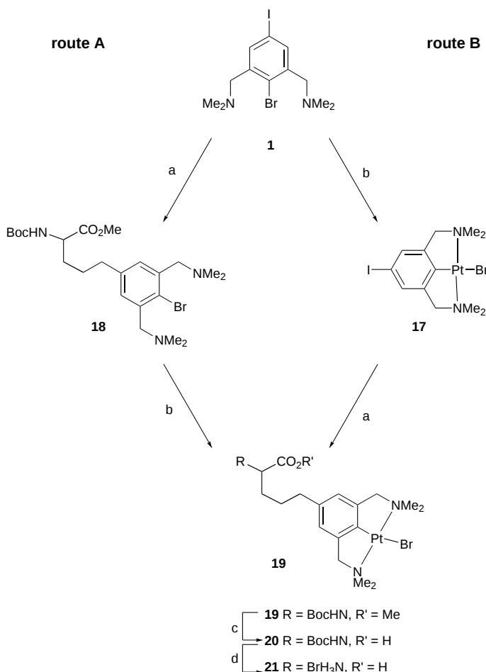
Scheme 7. Synthesis of an \alpha -amino acid labeled at the \alpha -carbon. Reagents and conditions: a) Boc-allylOMe, 9-BBN, THF, 2 h RT, then K 3 PO 4 , DMF, 10% [PdCl 2 (dppf)], 1 , \Delta , 12 h or K 3 PO 4 , DMF, 10% [PdCl 2 (dppf)], 17 , RT, 3 h; b) [Pt(4-tol) 2 (SEt 2 ) 2 ], C 6 H 6 , 50 °C, 3 h; c) LiOH, MeOH, RT, 12 h; d) HBr/Et 2 O, RT, 1 h.
