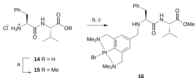
Scheme 6. Synthesis of a dipeptide labeled at the N terminus. Reagents and conditions: a) \text{SOCl}_2 , MeOH, \Delta , 1 h; b) 2 , \text{MgSO}_4 , Et 3 N, \text{CH}_2\text{Cl}_2 , RT, 12 h, then \text{NaBH}_3\text{CN} , HOAc, MeOH, 10 °C to RT, 2 h; c) [Pt(4-tol) 2 (SEt 2 ) 2 ], C 6 H 6 , 50 °C, 3 h.
