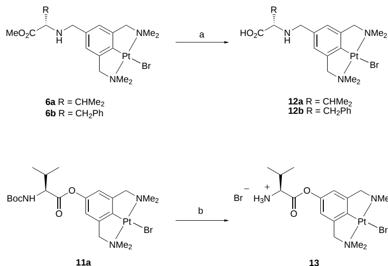
Scheme 5. Deprotection of \alpha -amino acids bound to platinum "pincer" markers. Reagents and conditions: a) LiOH, MeOH, RT, 12 h; b) HBr/AcOH or HBr/Et 2 O, RT, 1 h.
