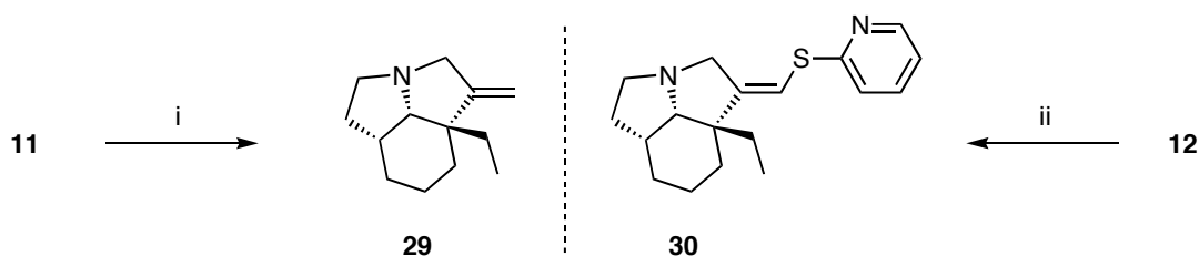
Scheme 5. Reagents and conditions: (i) n\text{-Bu}_3\text{SnH} (1 mol equiv.), AIBN (20 mol %), \text{C}_6\text{H}_6 , 80^\circ\text{C} , 5 h; (ii) malonic acid (3 mol equiv.) or \text{BF}_3\cdot\text{Et}_2\text{O} (3 mol equiv.), acetonitrile, irradiation, 0.5 h, ca. 18^\circ\text{C} .
