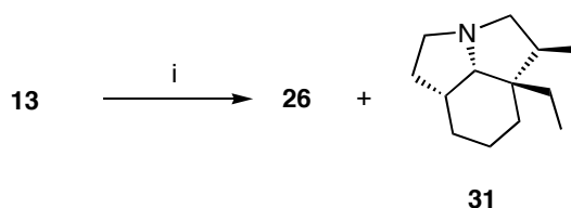
Scheme 6. Reagents and conditions: (i) n\text{-Bu}_3\text{SnH} (1.2 mol equiv.), AIBN (20 mol %), \text{C}_6\text{H}_6 , 80^\circ\text{C} , 6 h.
