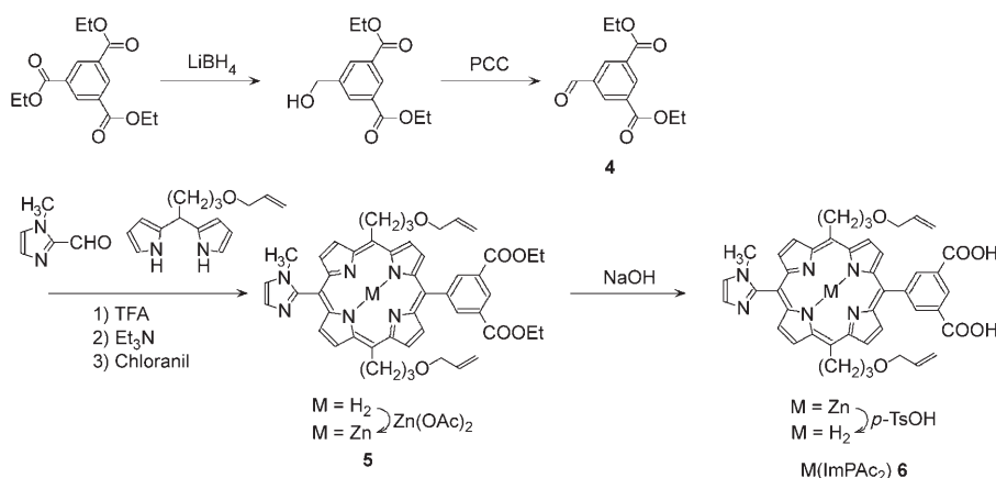
Scheme 5. Synthesis of H_2(\text{ImPAC}_2) ( 6 ).
