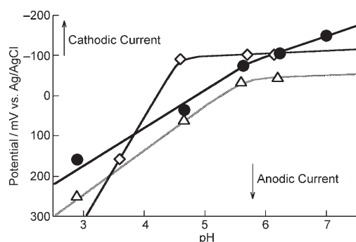
Figure 11. Plot of the apparent flat-band potential ( V_{fb} ) as a function of pH conditions for Zn(ImPPh)/Zn(ImPR)/ITO ( R = -PO_3 (●), -Ac_2 (◆), and -S_2 (△)).
