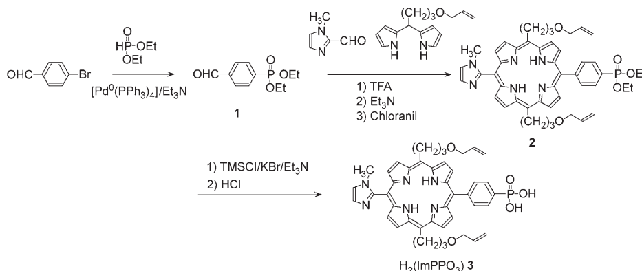
Scheme 4. Synthesis of \text{H}_2(\text{ImPPO}_3) ( 3 ).
