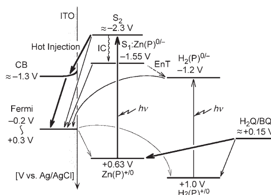
Scheme 3. Potential diagram for anodic photocurrent generation of \text{Zn}(\text{ImPPh})/\text{Zn}(\text{ImPPO}_3)/\text{ITO} by excitation at the Soret band in aqueous hydroquinone (50mM). Potentials are estimated based on refs.[14,34] and absorption spectra. The \text{S}_2 state of \text{H}_2(\text{ImPPO}_3) at -1.9 V is omitted for the sake of clarity.
