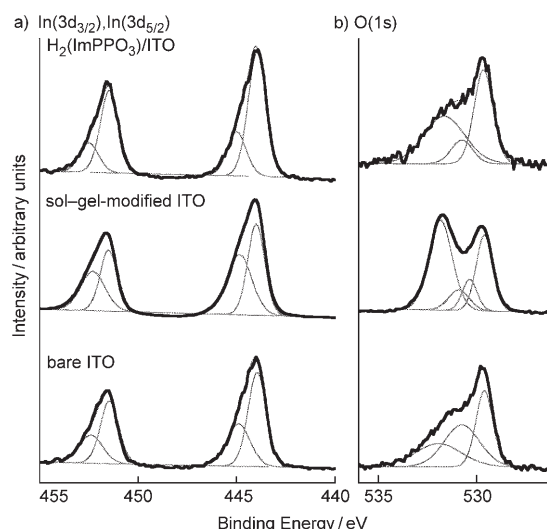
Figure 2. XPS-deconvoluted profiles of bare ITO, sol-gel-modified ITO, and \text{H}_2(\text{ImPPO}_3) -attached ITO (bottom to top) in the In(3d) region (a) and the O(1s) region (b) observed at a take-off angle of 60^\circ .
