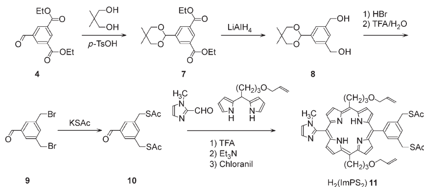
Scheme 6. Synthesis of H_2(ImPS_2) ( 11 ).
