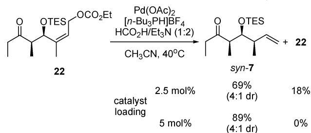
Scheme 2. Effect of Double-Bond Geometry
