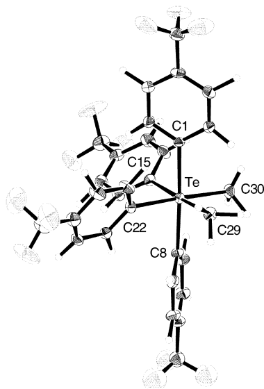
Figure 5. X-ray structure of cis - 4a (30% thermal ellipsoids). Selected bond lengths [Å]: Te–C1(aryl) 2.223(5), Te–C8(aryl) 2.208(5), Te–C15(aryl) 2.218(4), Te–C22(aryl) 2.217(4), Te–C29(methyl) 2.187(4), Te–C30(methyl) 2.185(4).
