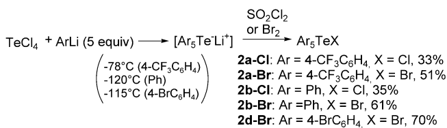
Scheme 3. Synthesis of pentaaryltellurium halides.
