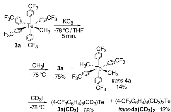
Scheme 6. Synthesis of trans - 4a by reduction of 3a with \text{KC}_8 followed by treatment with \text{CH}_3\text{I} (or \text{CD}_3\text{I} ).
