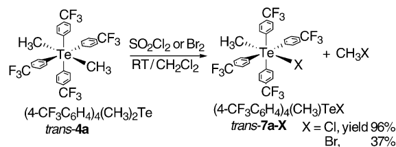
Scheme 15. Electrophilic halogenation of tetraaryl-dimethyltellurium.
