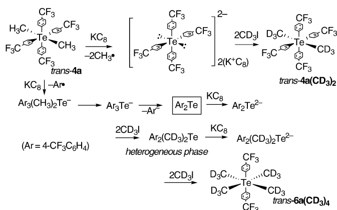
Scheme 9. Possible mechanism for formation of trans - 4a ( \text{CD}_3 ) 2 and trans - 6a ( \text{CD}_3 ) 4 in the reduction of trans - 4a with \text{KC}_8 followed by treatment with \text{CD}_3\text{I} .
