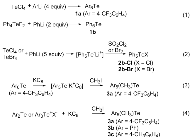
Scheme 1. Synthesis of hexavalent organotellurium compounds reported by us.
