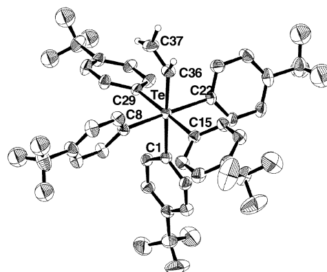
Figure 4. X-ray structure of 9 (30% thermal ellipsoids). Selected bond lengths [Å]: Te–C1(aryl) 2.238(5), Te–C8(aryl) 2.218(5), Te–C15(aryl) 2.213(5), Te–C22(aryl) 2.221(6), Te–C29(aryl) 2.221(5), Te–C36(vinyl) 2.177(5).
