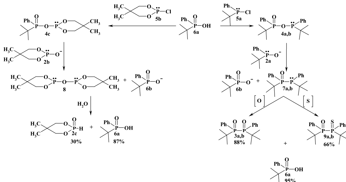
SCHEME 3 Reaction of \text{R}_2\text{P}-\text{O}^- ( 2 ) anions with mixed anhydrides \text{R}_2\text{P}(\text{O})-\text{O}-\text{PR}_2 ( 4 ).
