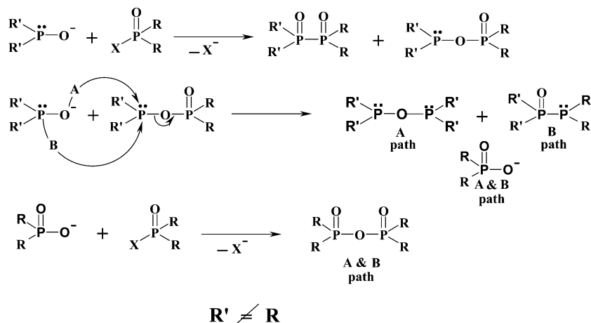
SCHEME 4 Mechanism proposed for the explanation of the origin of R_2P(O)-O-(O)PR_2 anhydride in the reaction mixture between >P-O^- nucleophiles and >P(O)X electrophiles ( X = Cl, Br ).
