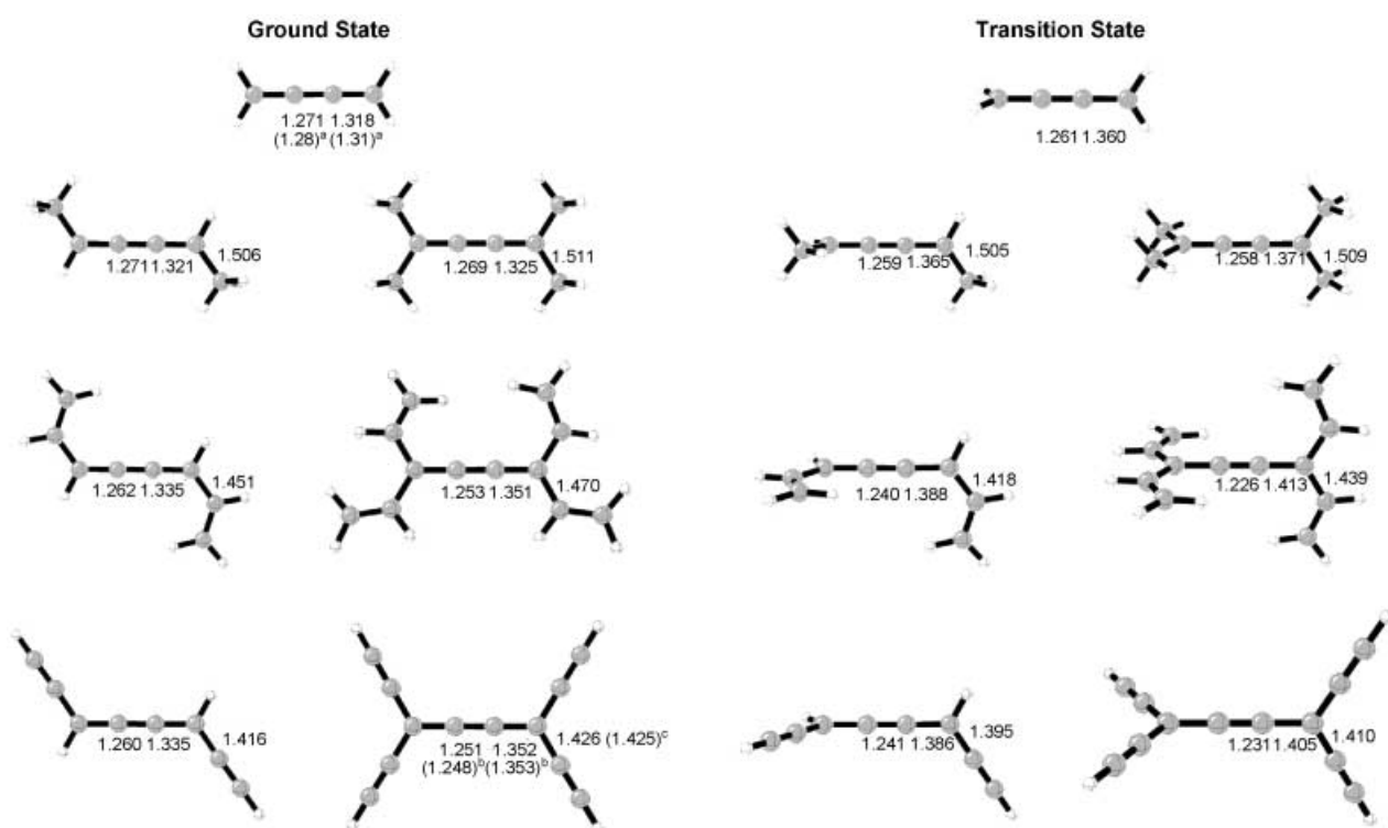
Figure 3. Ground- (left) and transition-state (right) geometries for butatriene, trans -1,4-dimethylbutatriene, tetramethylbutatriene, trans -1,4-diethynylbutatriene, tetraethynylbutatriene, and tetraethynylbutatriene. Unrestricted B3LYP6-31G(d) computed bond lengths \alpha , \beta , and \gamma are given along with experimental values in parentheses. a) See reference [22] for details. b) From the crystal structure analysis of the (\text{Me}_3\text{Si})_4 derivative in reference [8b]. c) Averaged bond lengths, see reference [8b].
