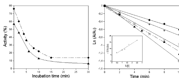
Fig. 1 (left) Residual enzymatic activity at different incubation times of inactivator 1 (residual concentration of 1 \blacklozenge 1 mM, \blacktriangle 2.2 mM); (right) k_{\text{obs}} determination at different inactivator concentrations ( \circ 2.2 mM, \blacktriangle 1 mM, \times 0.8 mM, \diamond 0.6 mM, \blacklozenge 0.4 mM); (inset) double reciprocal plot of k_{\text{obs}} versus concentration of 1 .
